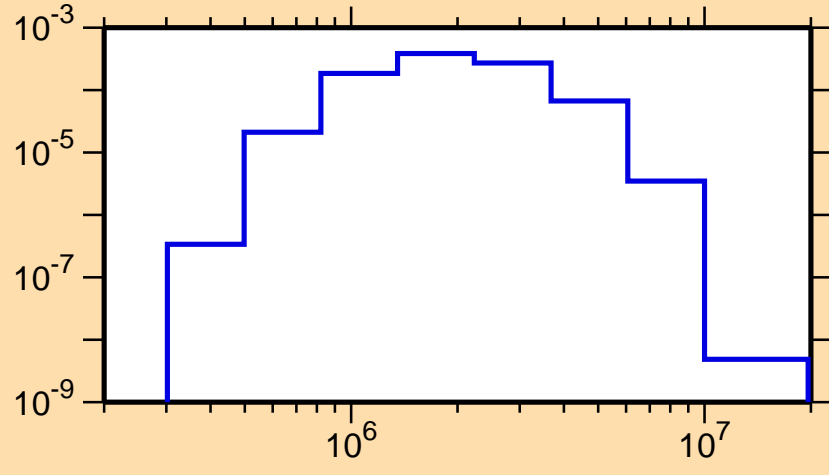
\sigma vs. E for ^{144}\text{Tb}(n,n_4)
