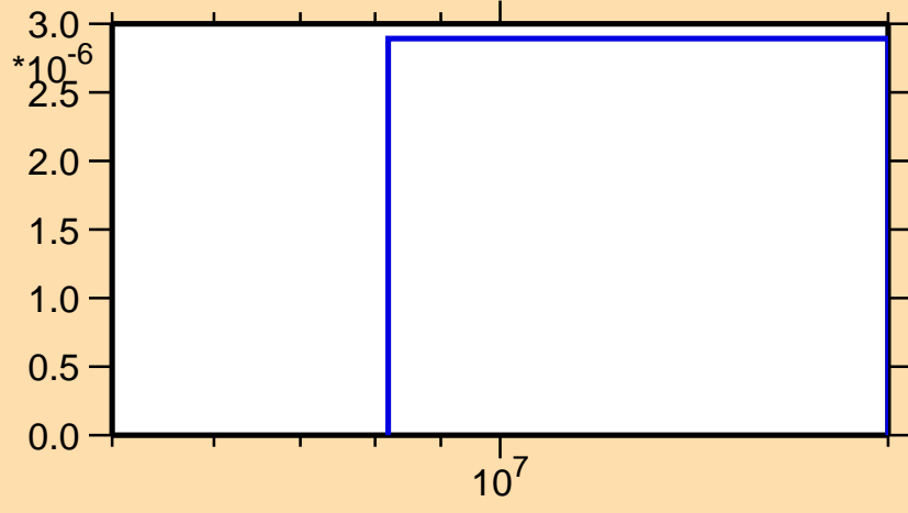
\sigma vs. E for ^{144}\text{Tb}(n,\text{nd})
