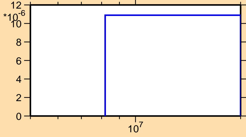
\sigma vs. E for ^{144}\text{Tb}(n,\text{pd})
