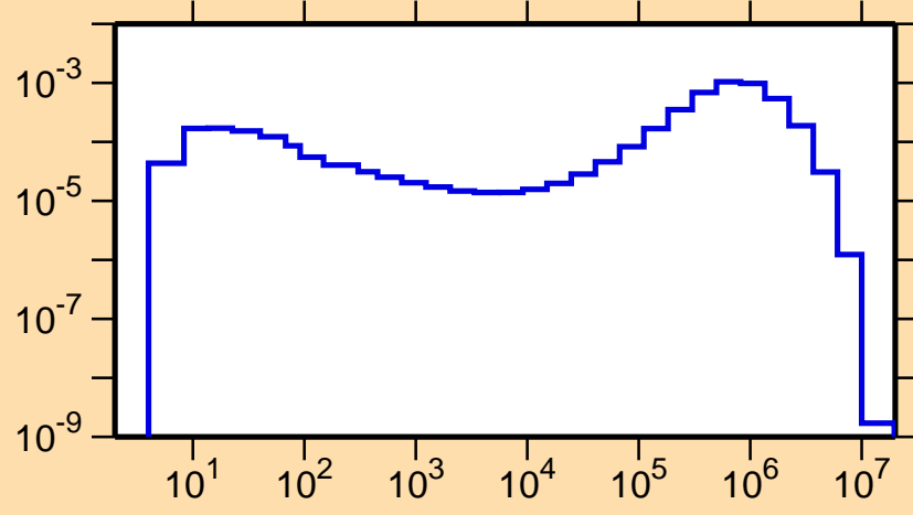
\sigma vs. E for ^{144}\text{Tb}(n,n_3)
