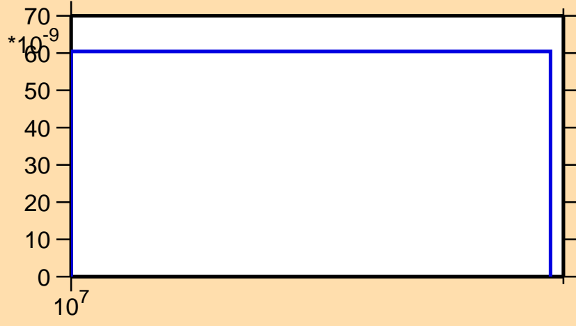
\sigma vs. E for ^{144}\text{Tb}(n,2n\alpha)
