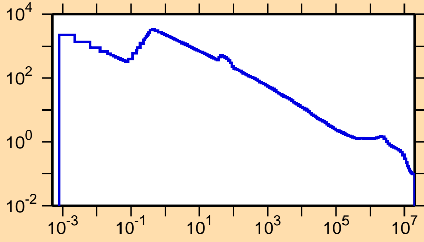
\sigma vs. E for ^{146}\text{Tb}(n,p)
