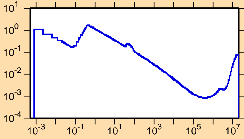
\sigma vs. E for ^{146}\text{Tb}(n,\alpha)
