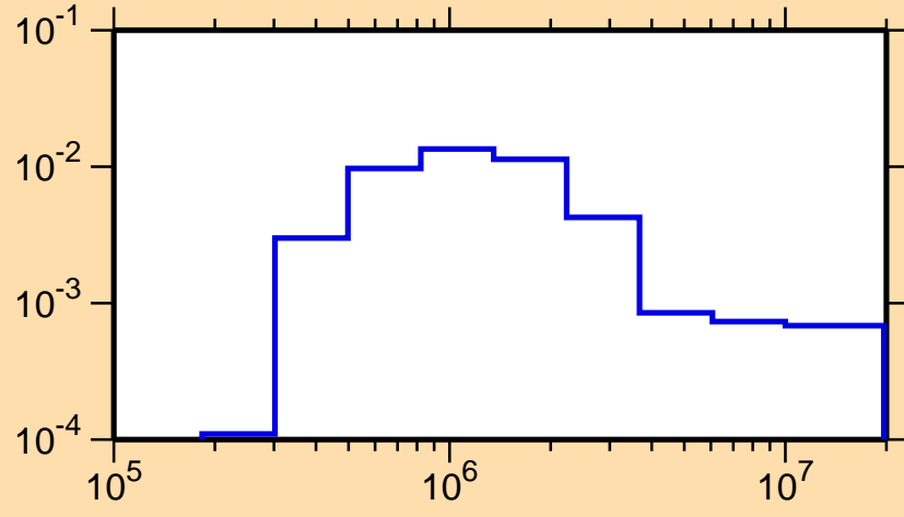
\sigma vs. E for ^{146}\text{Tb}(n,n_2)
