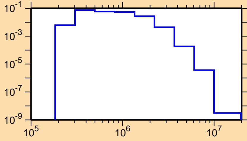
\sigma vs. E for ^{146}\text{Tb}(n,n_3)
