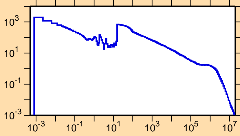
\sigma vs. E for ^{146}\text{Tb}(n,\gamma)
