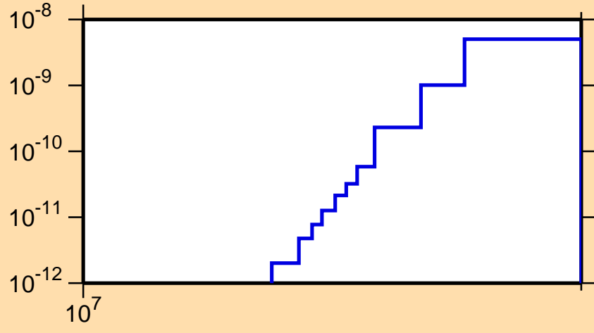
\sigma vs. E for ^{146}\text{Tb}(\text{mt117})
