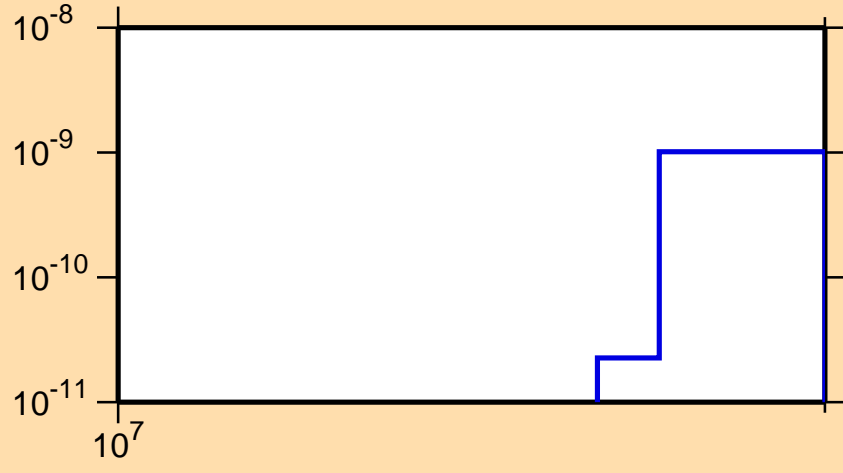
\sigma vs. E for ^{146}\text{Tb} (mt 34)
