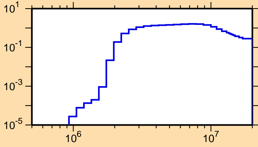
\sigma vs. E for ^{146}\text{Tb}(n,n\text{cont.})
