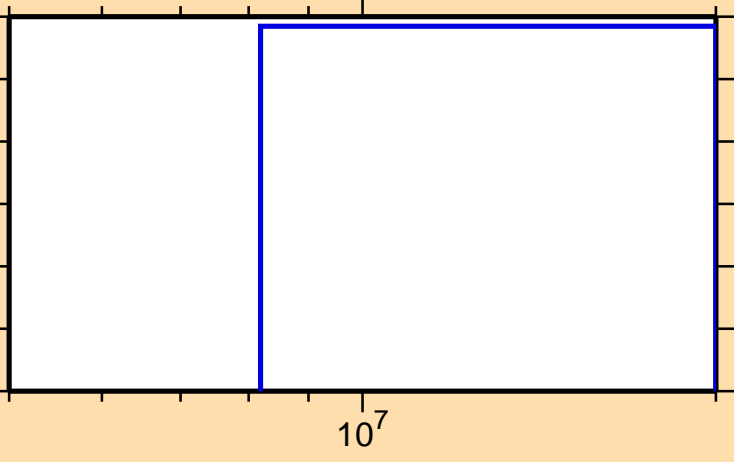
\sigma vs. E for ^{146}\text{Tb}(\text{mt117})
