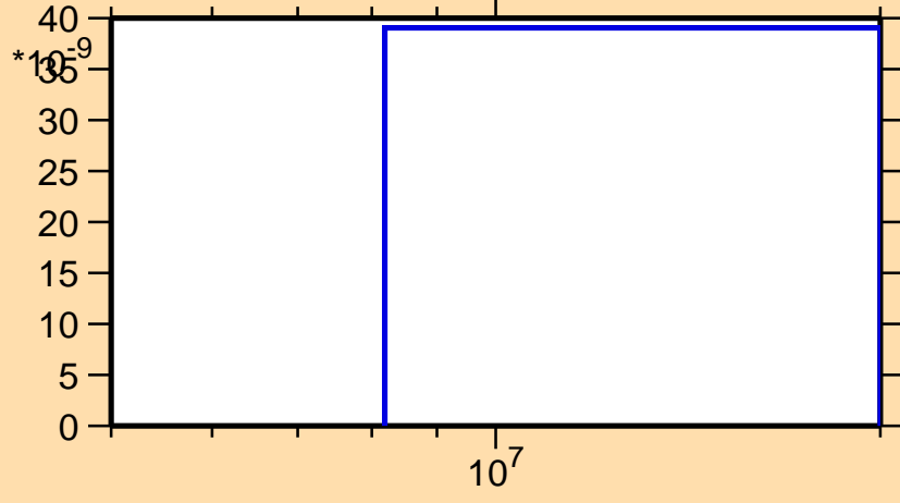
\sigma vs. E for ^{147}\text{Tb} (mt 45)
