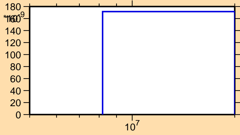
\sigma vs. E for ^{147}\text{Tb}(n,pd)
