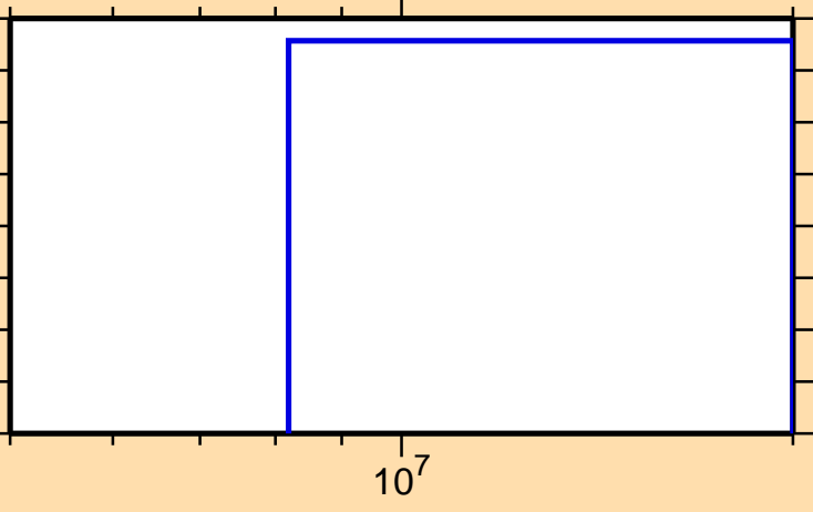
\sigma vs. E for ^{147}\text{Tb}(n,2np)
