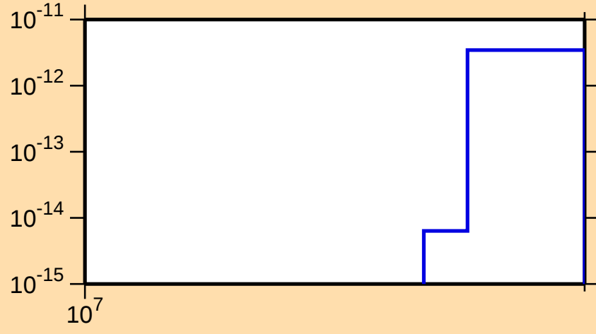
\sigma vs. E for ^{147}\text{Tb}(\text{mt } 34)
