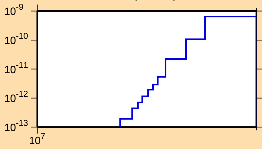
\sigma vs. E for ^{147}\text{Tb}(\text{mt117})
