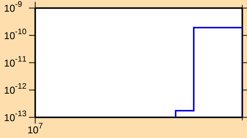
\sigma vs. E for ^{147}\text{Tb}(n,2n\alpha)
