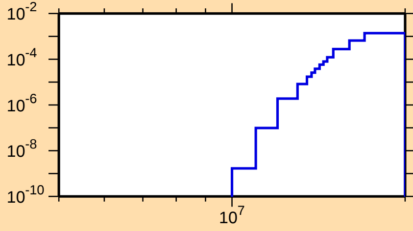
\sigma vs. E for ^{147}\text{Tb}(n,t)
