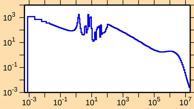
\sigma vs. E for ^{147}\text{Tb}(n,\gamma)
