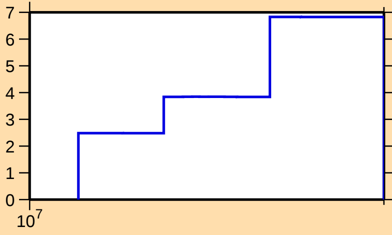
\Delta\sigma/\sigma vs. E for ^{147}\text{Tb}(n,\text{tot.})
