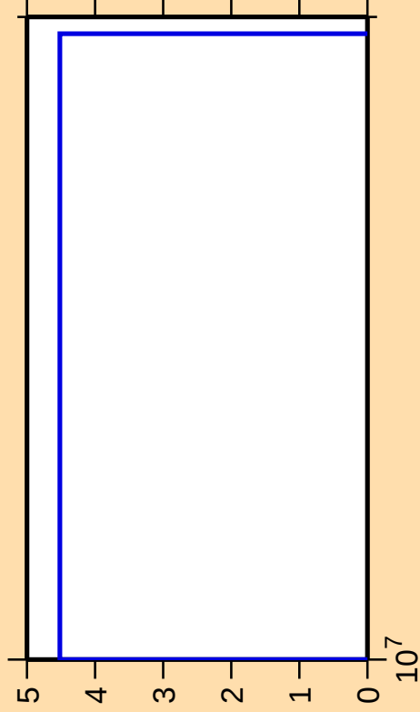
\Delta\sigma/\sigma vs. E for ^{147}\text{Tb}(n,\text{nt})
