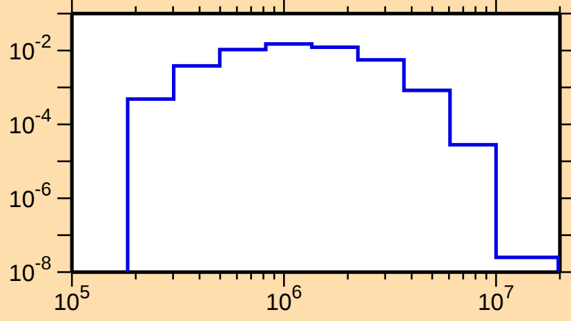
\sigma vs. E for ^{147}\text{Tb}(n,n_2)
