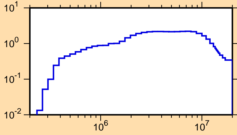
\sigma vs. E for ^{148}\text{Tb}(n,\text{inel.})
