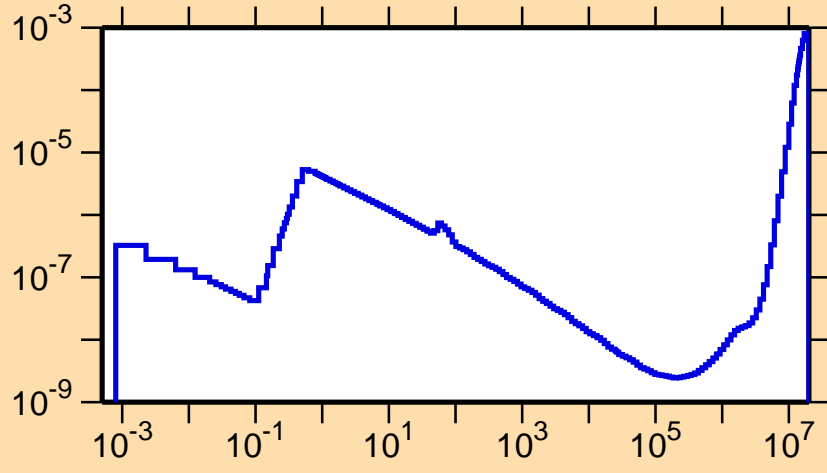
\sigma vs. E for ^{148}\text{Tb}(n,p\alpha)
