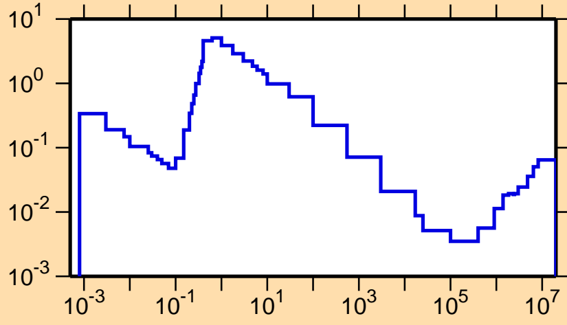
\sigma vs. E for ^{148}\text{Tb}(n,p)
