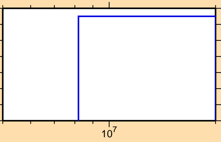
\sigma vs. E for ^{148}\text{Tb}(n,2np)
