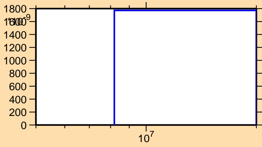
\sigma vs. E for ^{148}\text{Tb}(n,\text{nd})
