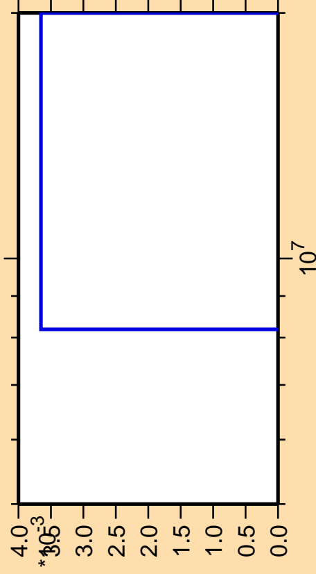
\Delta\sigma/\sigma vs. E for ^{149}\text{Tb}(\text{mt } 11)
