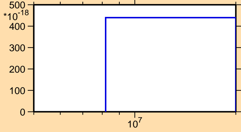
\sigma vs. E for ^{149}\text{Tb}(\text{mt } 11)
