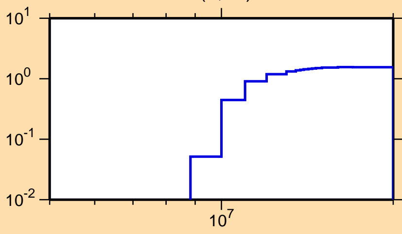
\sigma vs. E for ^{149}\text{Tb}(n,2n)
