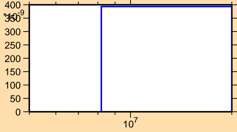
\sigma vs. E for ^{149}\text{Tb}(n,\text{He}3)
