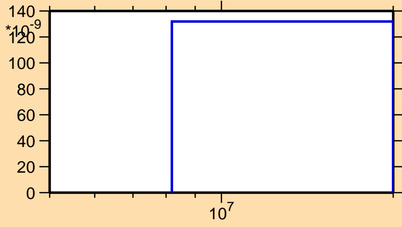
\sigma vs. E for ^{149}\text{Tb} (mt 45)
