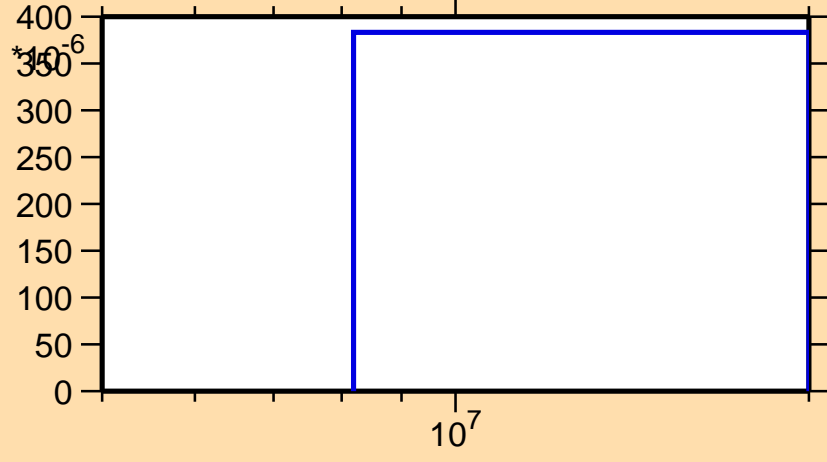
\sigma vs. E for ^{150}\text{Tb}(n,3n)
