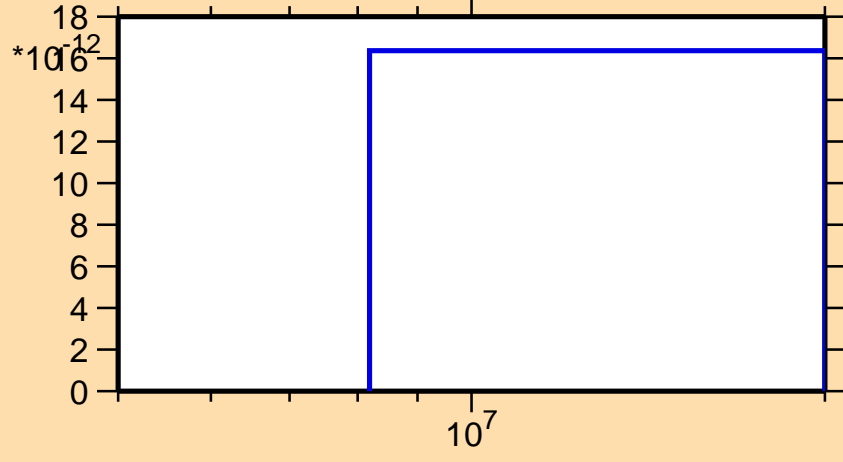
\sigma vs. E for ^{150}\text{Tb}(n,pd)
