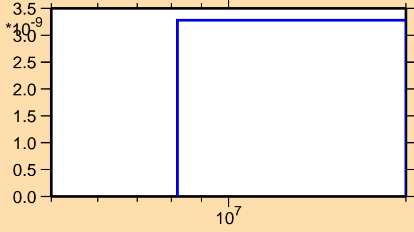
\sigma vs. E for ^{150}\text{Tb}(\text{mt117})
