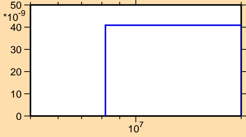
\sigma vs. E for ^{150}\text{Tb} (mt 45)
