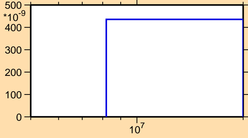
\sigma vs. E for ^{150}\text{Tb}(n,\text{He}3)
