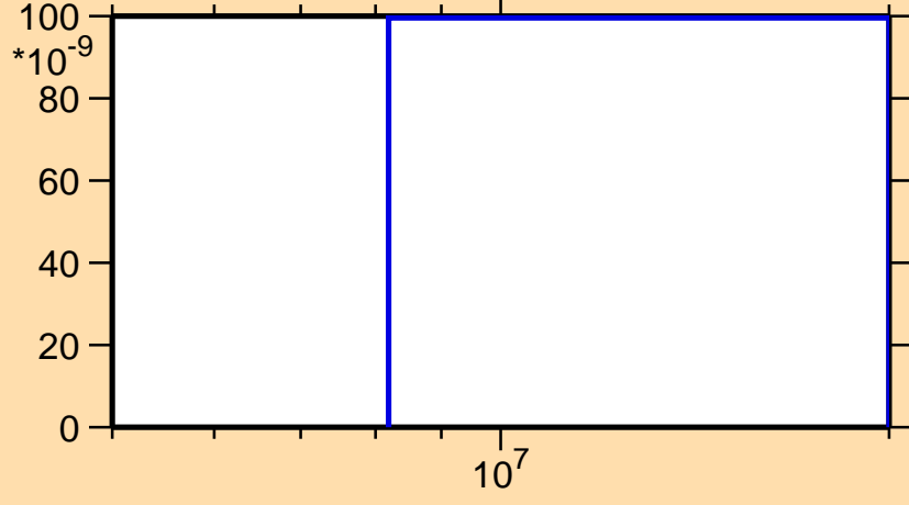
\sigma vs. E for ^{150}\text{Tb}(n,nt)
