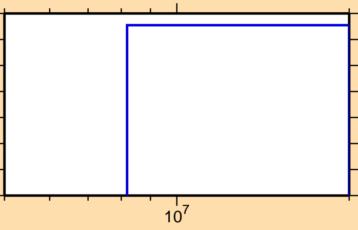
\sigma vs. E for ^{150}\text{Tb}(n,2np)
