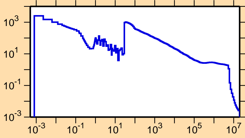
\sigma vs. E for ^{150}\text{Tb}(n,\gamma)
