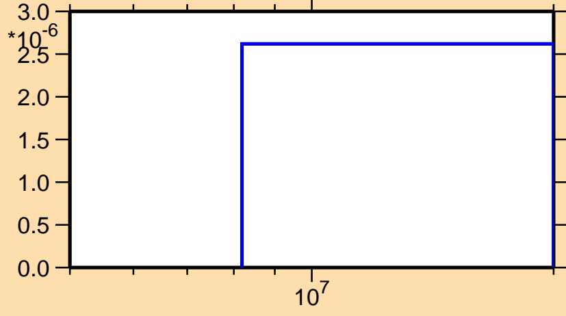
\sigma vs. E for ^{150}\text{Tb}(n,\text{nd})
