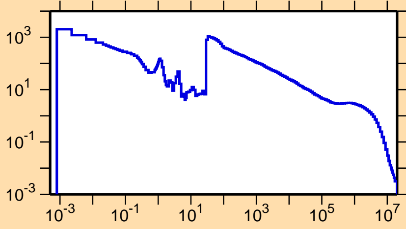
\sigma vs. E for ^{151}\text{Tb}(n,\gamma)
