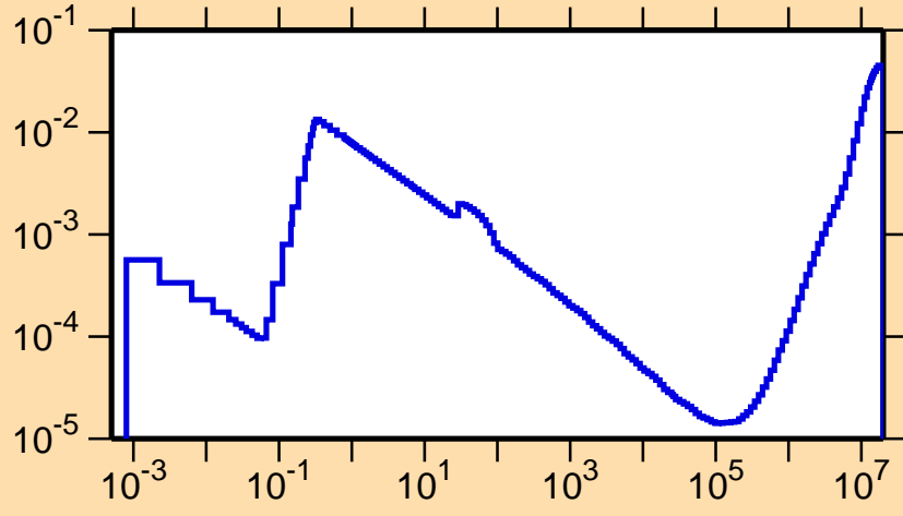
\sigma vs. E for ^{151}\text{Tb}(n,p)
