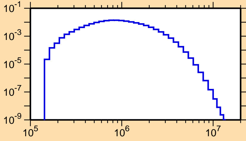
\sigma vs. E for ^{151}\text{Tb}(n,n_4)
