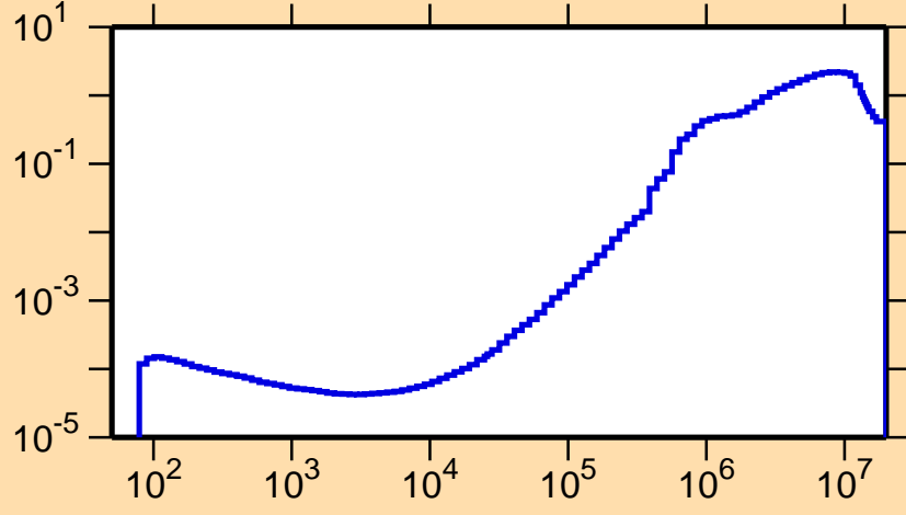
\sigma vs. E for ^{151}\text{Tb}(n,\text{inel.})
