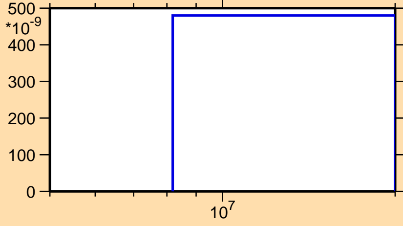
\sigma vs. E for ^{151}\text{Tb}(n,\text{nd})
