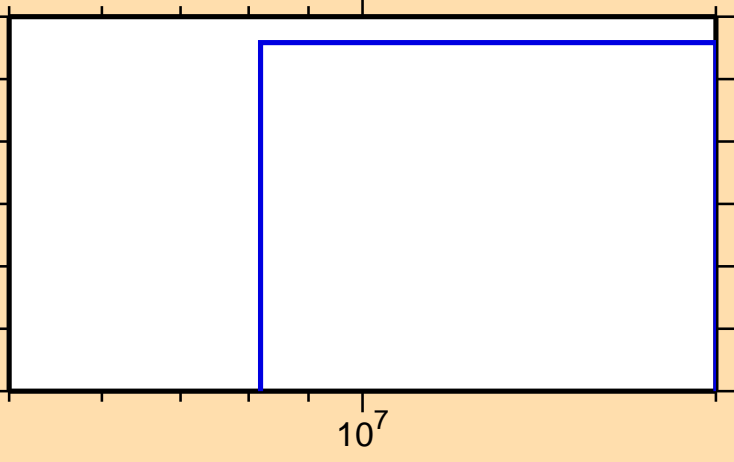
\sigma vs. E for ^{151}\text{Tb} (mt 34)
