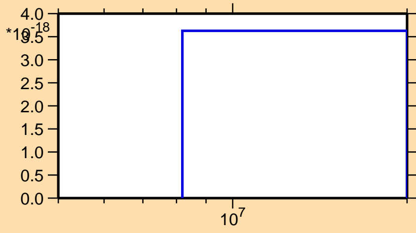
\sigma vs. E for ^{151}\text{Tb} (mt 42)
