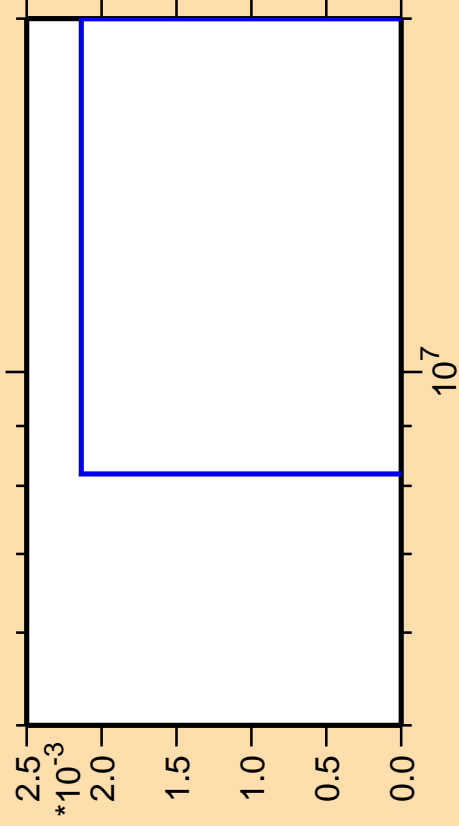
\Delta\sigma/\sigma vs. E for ^{151}\text{Tb}(\text{mt } 11)
