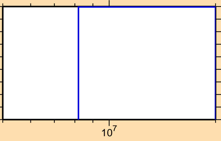
\sigma vs. E for ^{152}\text{Tb}(n,\text{pt})
