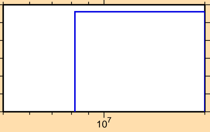
\sigma vs. E for ^{152}\text{Tb}(n,\text{nd})
