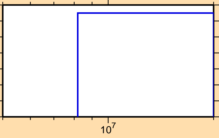
\sigma vs. E for ^{152}\text{Tb}(n,nt)
