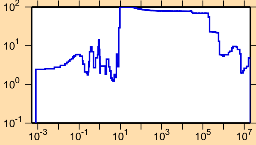
\Delta\sigma/\sigma vs. E for ^{152}\text{Tb}(n,el.)
