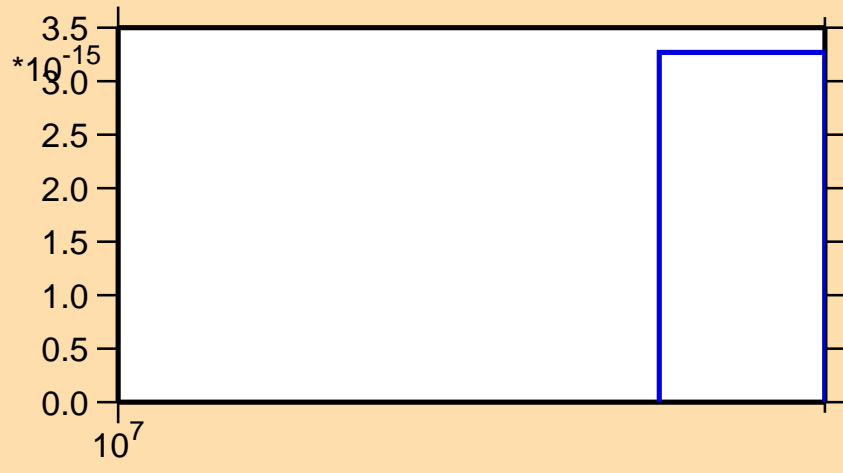
\sigma vs. E for ^{152}\text{Tb} (mt 42)
