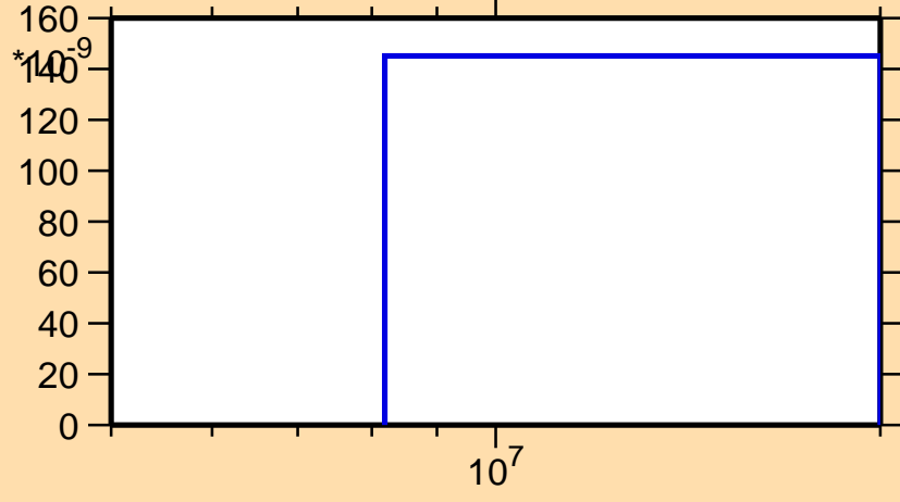
\sigma vs. E for ^{152}\text{Tb}(n,nt)
