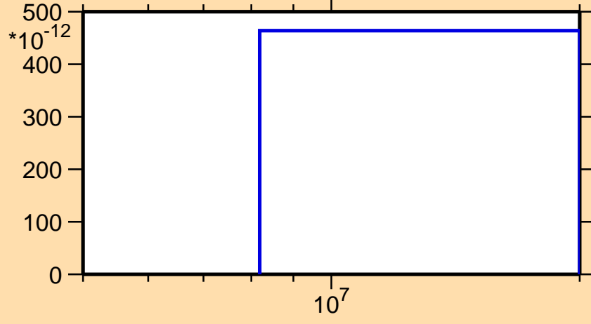
\sigma vs. E for ^{152}\text{Tb} (mt 45)
