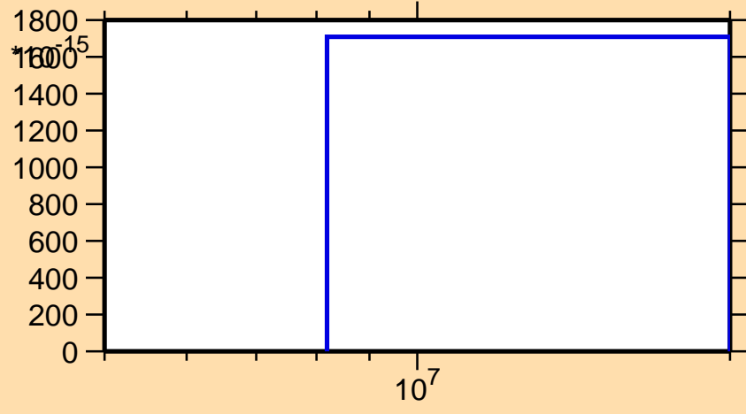
\sigma vs. E for ^{152}\text{Tb} (mt 34)
