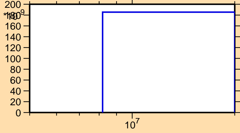
\sigma vs. E for ^{152}\text{Tb}(n,3n\alpha)
