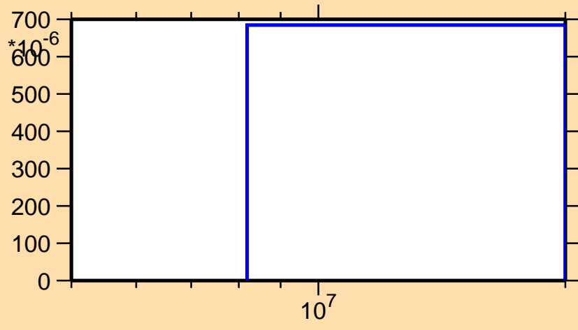
\sigma vs. E for ^{152}\text{Tb}(n,3n)
