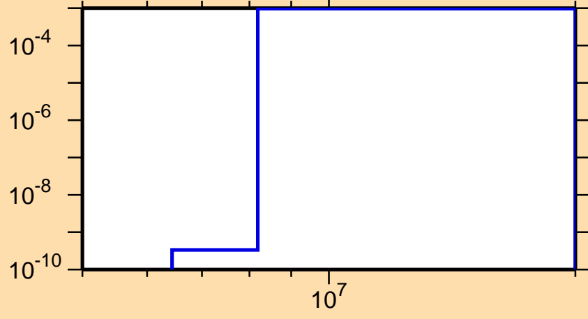
\sigma vs. E for ^{152}\text{Tb}(n,t)
