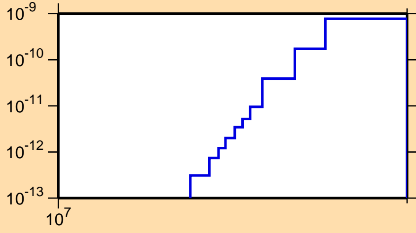
\sigma vs. E for ^{153}\text{Tb}(\text{mt117})
