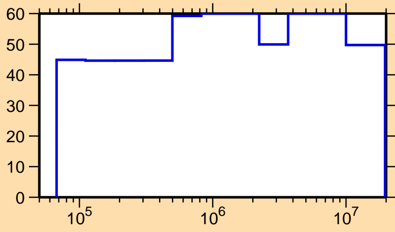
\Delta\sigma/\sigma vs. E for ^{153}\text{Tb}(n,n_1)
