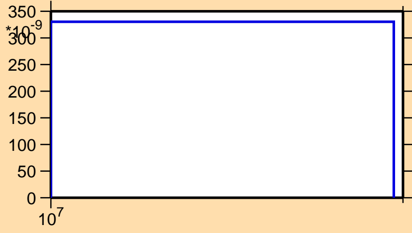
\sigma vs. E for ^{153}\text{Tb}(n,\text{nd})
