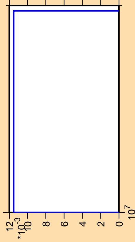
\Delta\sigma/\sigma vs. E for ^{153}\text{Tb} (mt 34)
