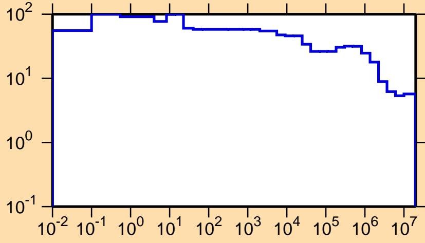
\Delta\sigma/\sigma vs. E for ^{153}\text{Tb}(n,\text{nonel.})
