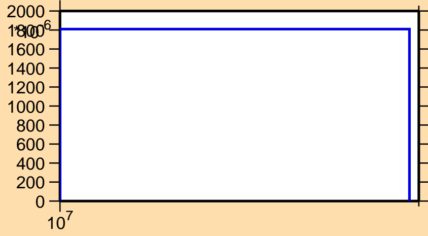
\sigma vs. E for ^{153}\text{Tb}(n,3n)
