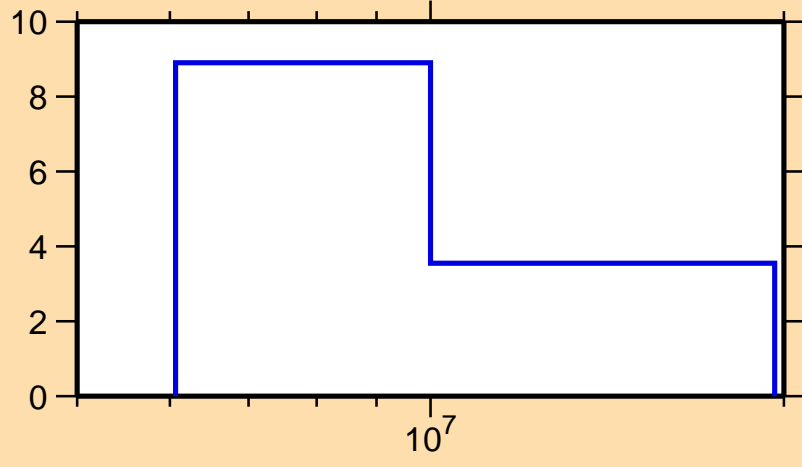
\Delta\sigma/\sigma vs. E for ^{153}\text{Tb}(n,\text{tot.})
