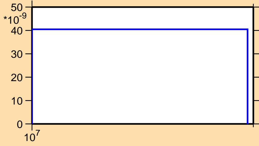
\sigma vs. E for ^{153}\text{Tb}(n,nt)
