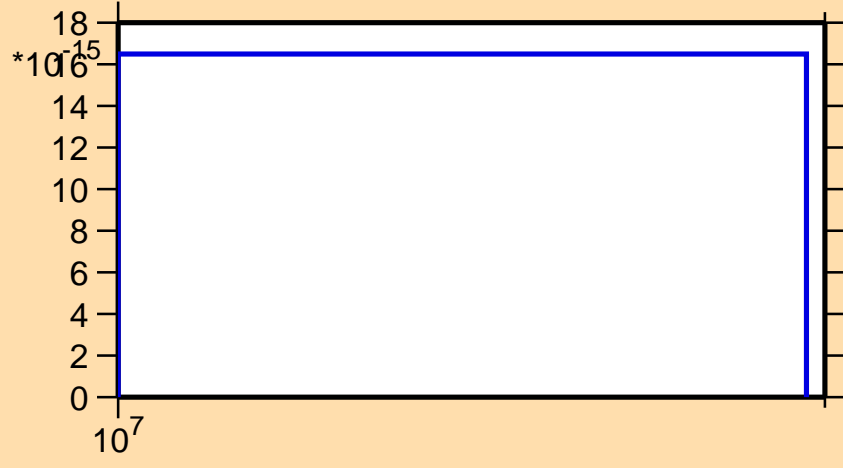
\sigma vs. E for ^{153}\text{Tb}(n,pd)
