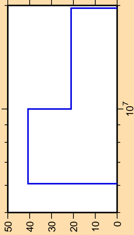
\Delta\sigma/\sigma vs. E for ^{153}\text{Tb}(n,2n)
