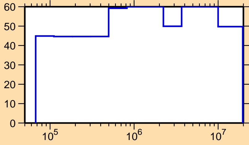
\Delta\sigma/\sigma vs. E for ^{153}\text{Tb}(n,n_1)
