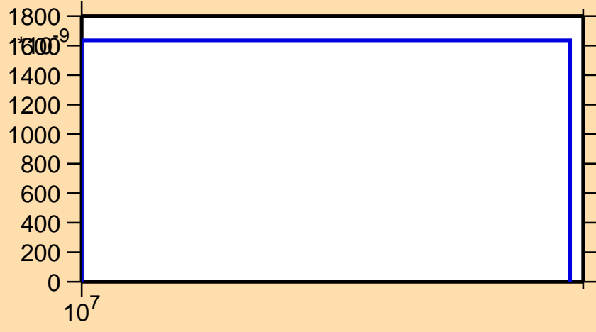
\sigma vs. E for ^{153}\text{Tb}(n,2np)
