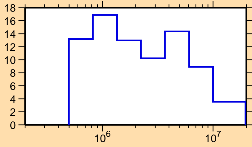
\Delta\sigma/\sigma vs. E for ^{153}\text{Tb}(n,\text{tot.})
