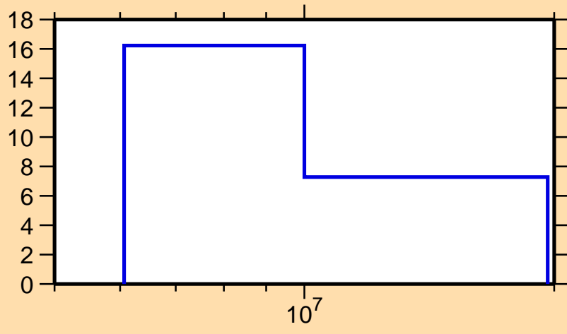
\Delta\sigma/\sigma vs. E for ^{153}\text{Tb}(n,\text{el.})
