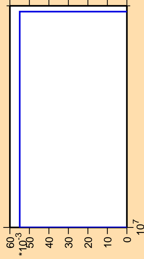
\Delta\sigma/\sigma vs. E for ^{153}\text{Tb}(n,pd)
