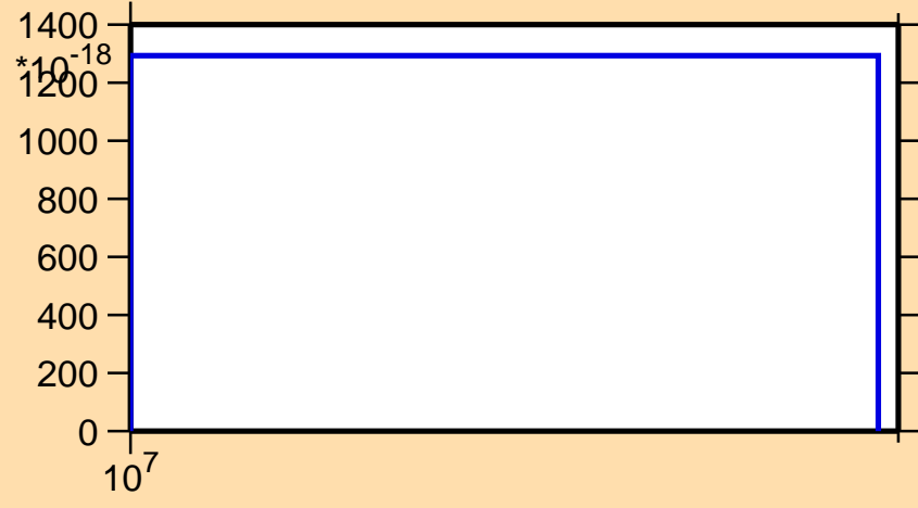
\sigma vs. E for ^{153}\text{Tb} (mt 34)
