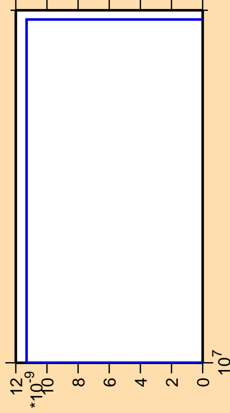
\Delta\sigma/\sigma vs. E for ^{153}\text{Tb} (mt 42)
