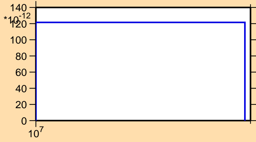
\sigma vs. E for ^{153}\text{Tb} (mt 45)
