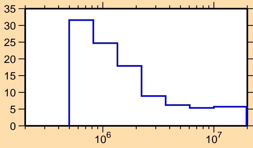
\Delta\sigma/\sigma vs. E for ^{153}\text{Tb}(n,\text{nonel.})
