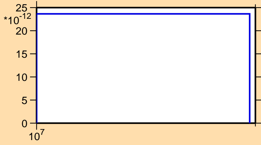
\sigma vs. E for ^{153}\text{Tb}(\text{mt117})
