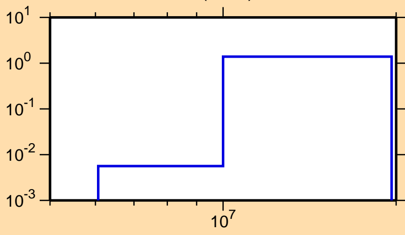
\sigma vs. E for ^{153}\text{Tb}(n,2n)
