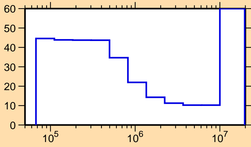
\Delta\sigma/\sigma vs. E for ^{153}\text{Tb}(n,\text{inel.})
