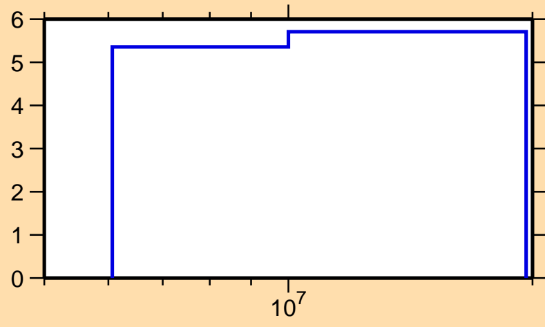
\Delta\sigma/\sigma vs. E for ^{153}\text{Tb}(n,\text{nonel.})
