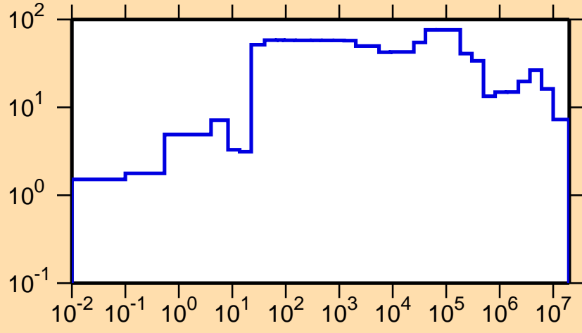
\Delta\sigma/\sigma vs. E for ^{153}\text{Tb}(n,\text{el.})
