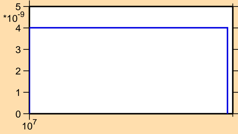
\sigma vs. E for ^{153}\text{Tb}(n,\text{He3})
