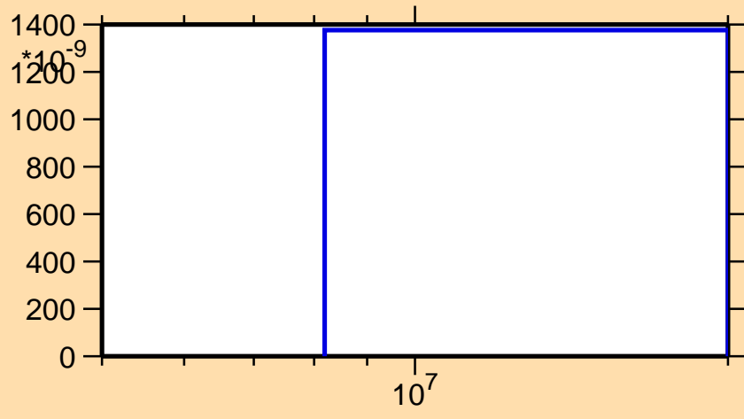
\sigma vs. E for ^{153}\text{Tb}(n,2np)
