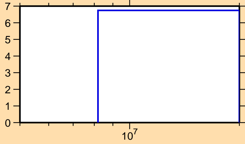
\Delta\sigma/\sigma vs. E for ^{153}\text{Tb}(n,\text{el.})
