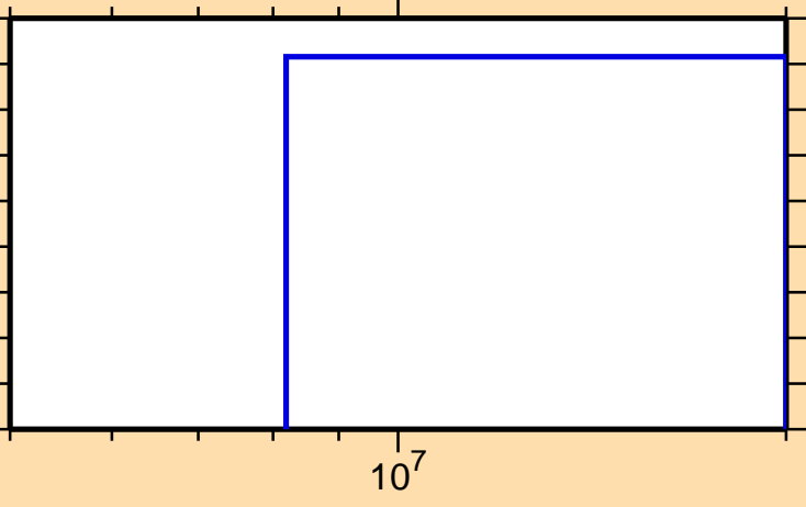
\sigma vs. E for ^{153}\text{Tb}(n,pd)
