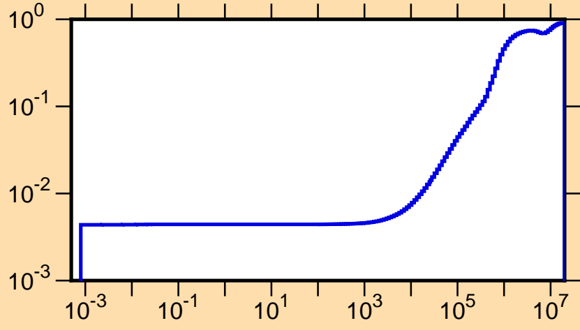
\mu vs. E for ^{154}\text{Tb}(\text{mt251})
