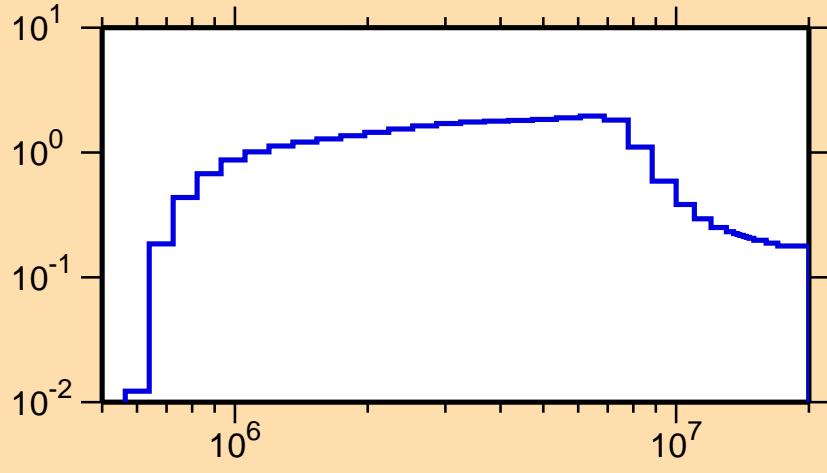
\sigma vs. E for ^{154}\text{Tb}(n,n\text{cont.})
