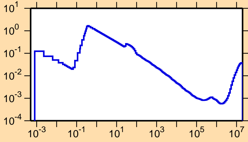
\sigma vs. E for ^{154}\text{Tb}(n,p)
