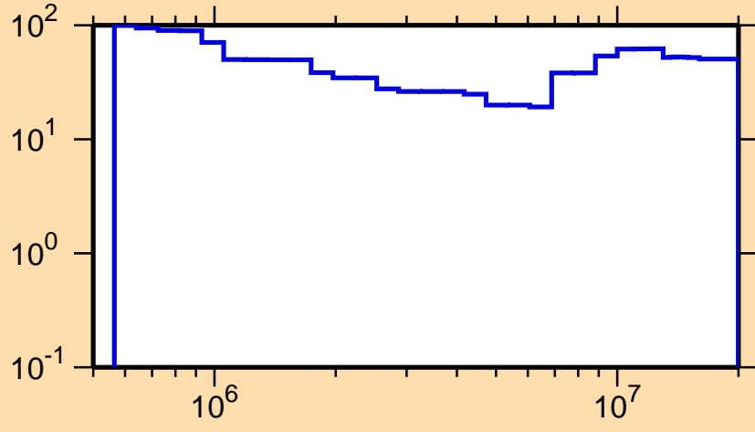
\Delta\sigma/\sigma vs. E for ^{154}\text{Tb}(n,n\text{cont.})
