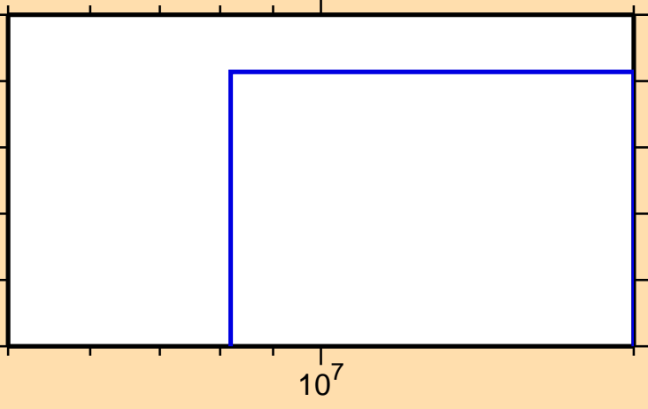
\sigma vs. E for ^{154}\text{Tb}(n,2np)
