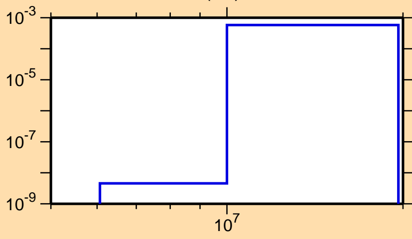
\sigma vs. E for ^{154}\text{Tb}(n,t)
