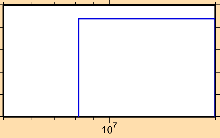
\sigma vs. E for ^{154}\text{Tb}(n,\text{He3})
