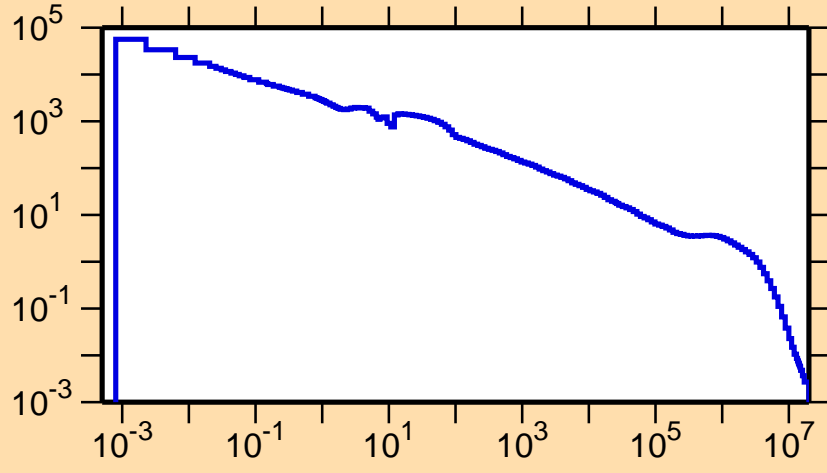
\sigma vs. E for ^{154}\text{Tb}(n,\gamma)
