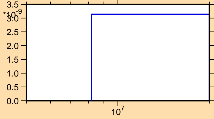
\sigma vs. E for ^{154}\text{Tb}(n,p\alpha)
