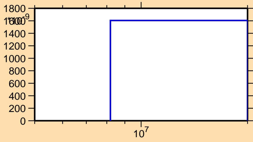
\sigma vs. E for ^{154}\text{Tb}(n,\text{nd})
