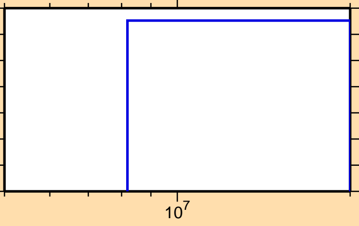
\sigma vs. E for ^{154}\text{Tb}(\text{mt117})
