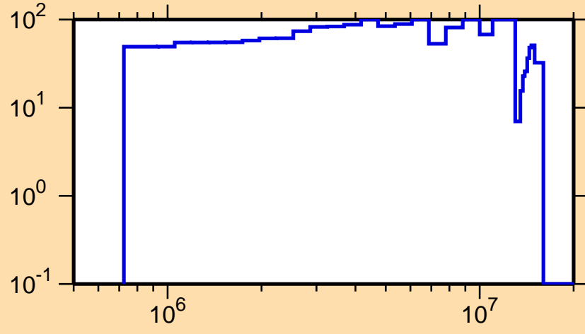
\Delta\sigma/\sigma vs. E for ^{155}\text{Tb}(n,n_1)
