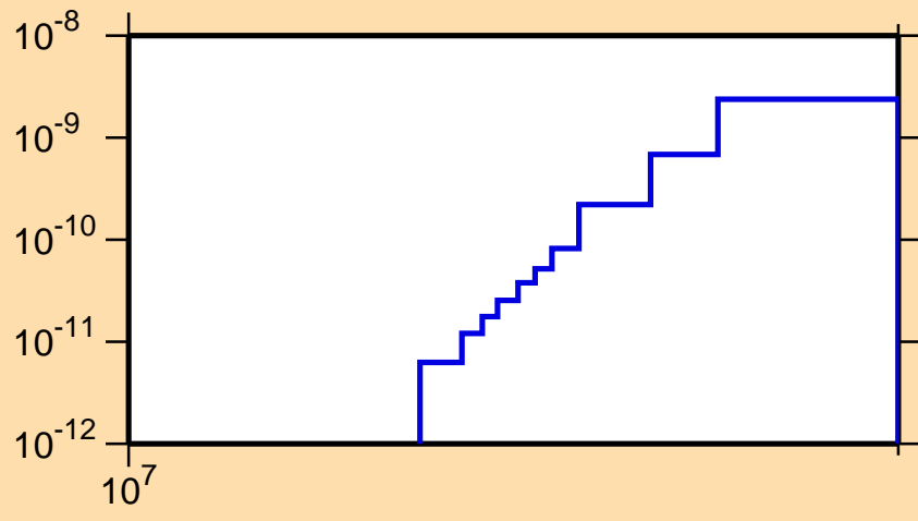
\sigma vs. E for ^{155}\text{Tb}(n,p\alpha)
