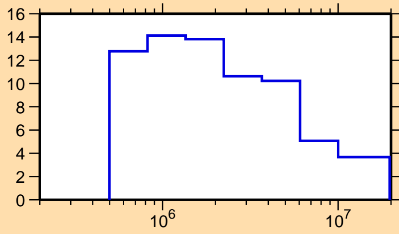
\Delta\sigma/\sigma vs. E for ^{155}\text{Tb}(n,\text{tot.})
