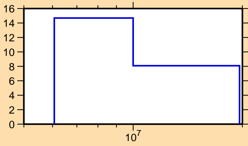
\Delta\sigma/\sigma vs. E for ^{155}\text{Tb}(n,\text{el.})
