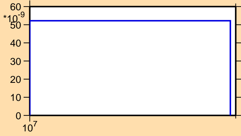
\sigma vs. E for ^{155}\text{Tb}(n,2np)
