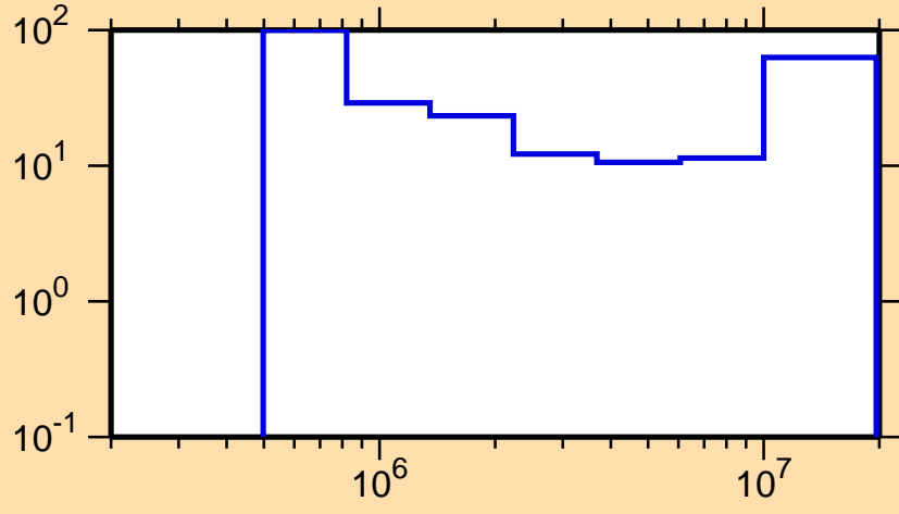
\Delta\sigma/\sigma vs. E for ^{155}\text{Tb}(n,n\text{cont.})
