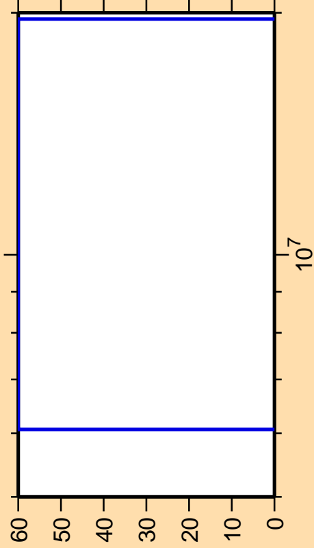
\Delta\sigma/\sigma vs. E for ^{155}\text{Tb}(n,np)
