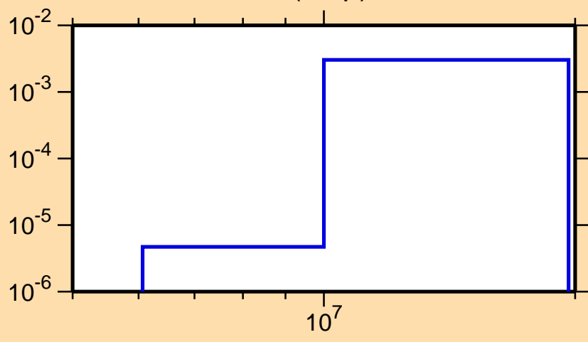
\sigma vs. E for ^{155}\text{Tb}(n,np)
