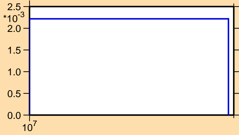
\sigma vs. E for ^{155}\text{Tb}(n,3n)
