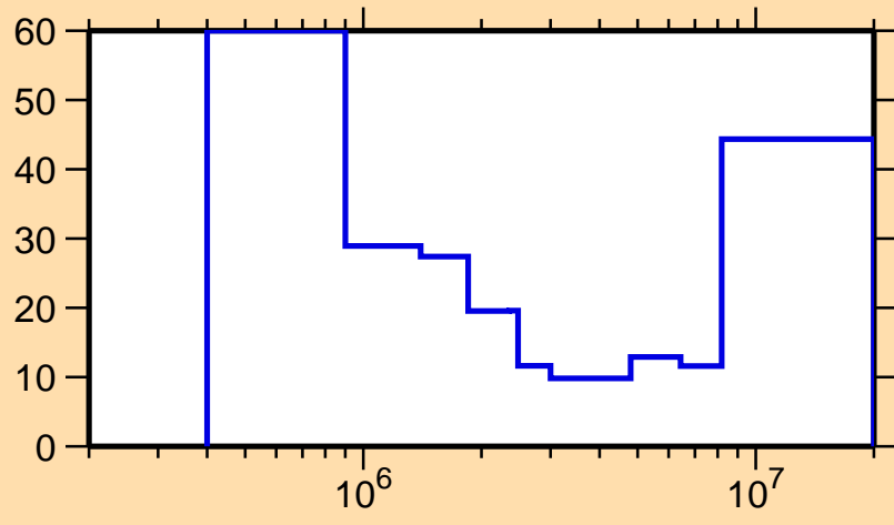
\Delta\sigma/\sigma vs. E for ^{155}\text{Tb}(n,n\text{cont.})
