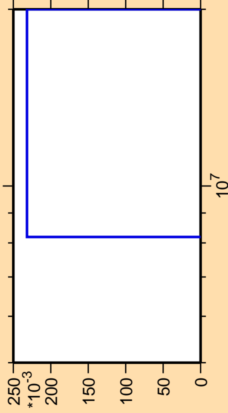
\Delta\sigma/\sigma vs. E for ^{155}\text{Tb}(\text{mt } 45)
