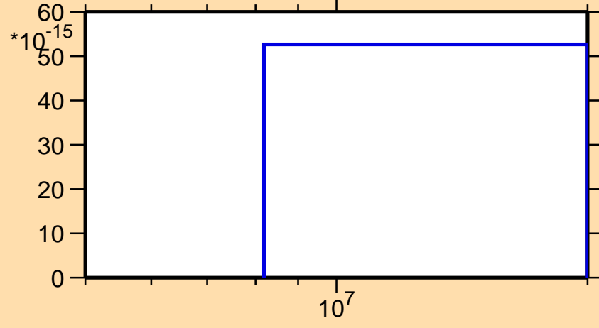
\sigma vs. E for ^{155}\text{Tb}(\text{mt } 45)
