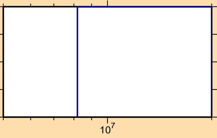
\sigma vs. E for ^{155}\text{Tb}(n,\text{He3})
