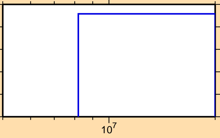
\sigma vs. E for ^{156}\text{Tb}(n,nt)
