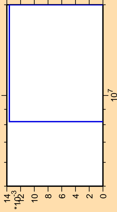
\Delta\sigma/\sigma vs. E for ^{156}\text{Tb} (mt 45)
