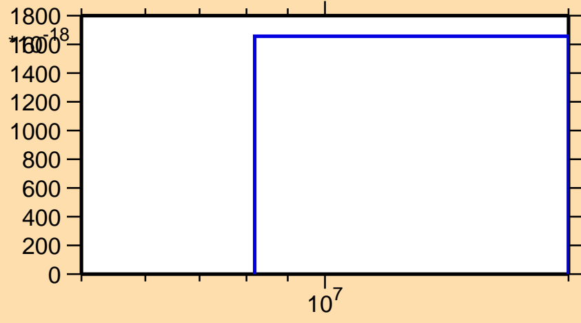
\sigma vs. E for ^{156}\text{Tb} (mt 45)
