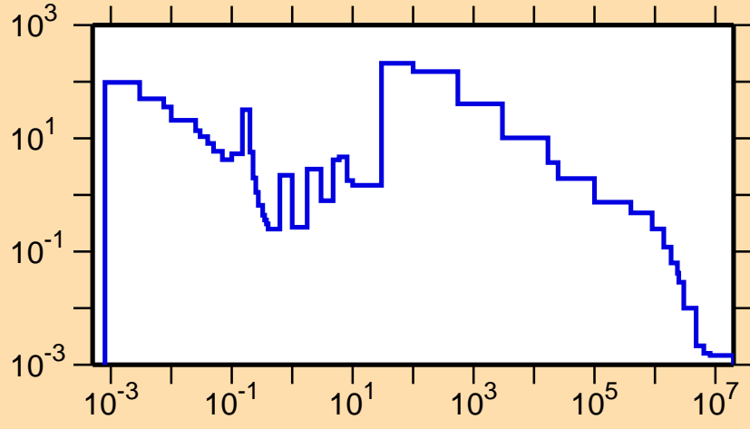
\sigma vs. E for ^{156}\text{Tb}(n,\gamma)
