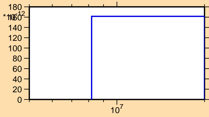
\sigma vs. E for ^{156}\text{Tb}(n,p\alpha)
