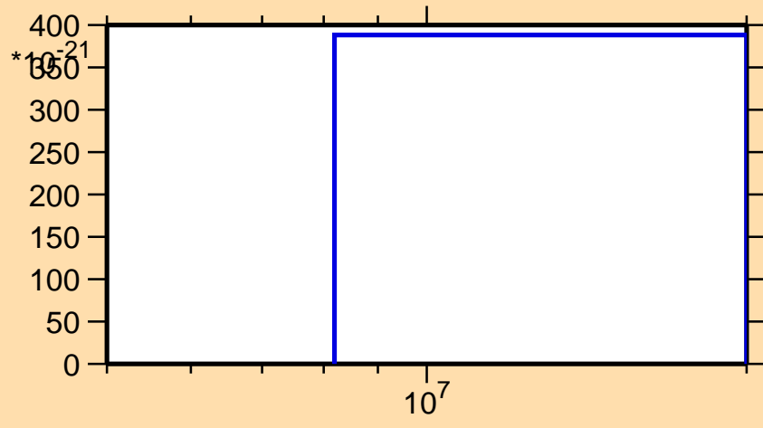
\sigma vs. E for ^{156}\text{Tb}(\text{mt } 11)
