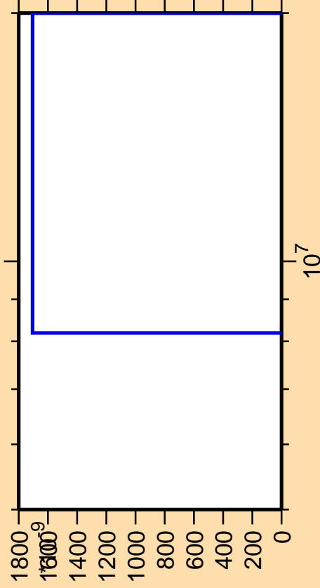
\Delta\sigma/\sigma vs. E for ^{156}\text{Tb}(\text{mt } 11)
