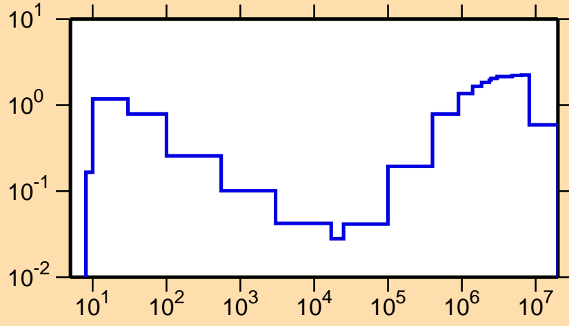
\sigma vs. E for ^{156}\text{Tb}(n,\text{inel.})
