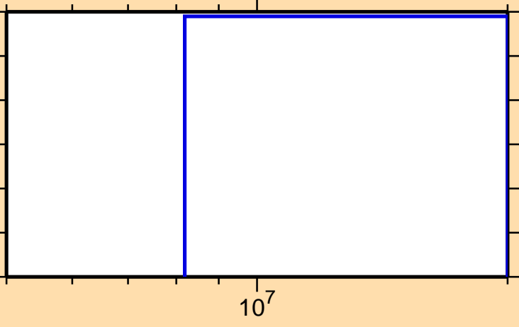
\sigma vs. E for ^{156}\text{Tb}(n,\text{He3})
