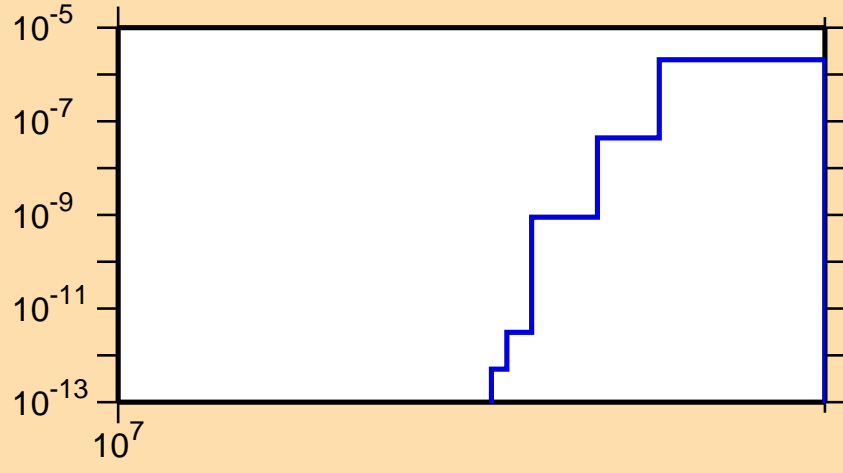
\sigma vs. E for ^{157}\text{Tb}(n,\text{nd})
