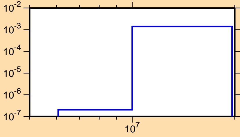
\sigma vs. E for ^{157}\text{Tb}(n,np)
