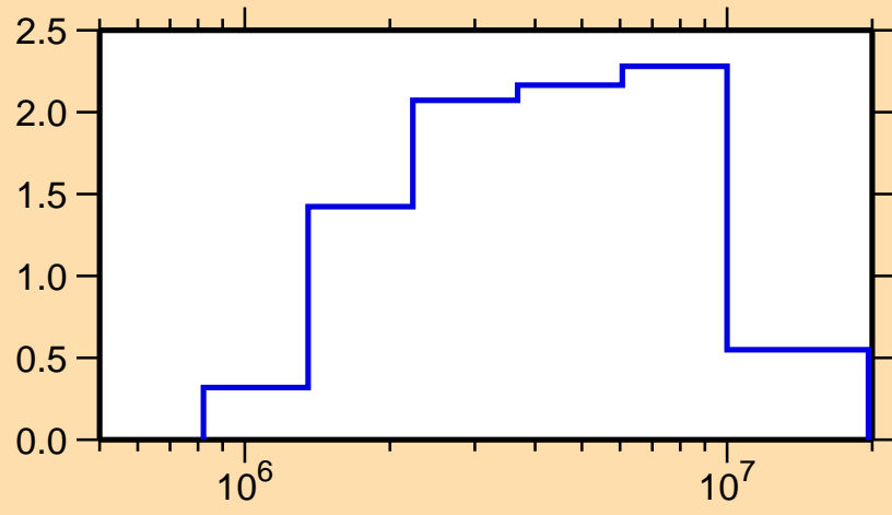
\sigma vs. E for ^{157}\text{Tb}(n,n\text{cont.})
