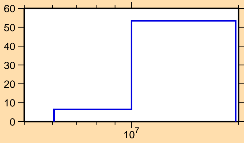
\Delta\sigma/\sigma vs. E for ^{157}\text{Tb}(n,\text{inel.})
