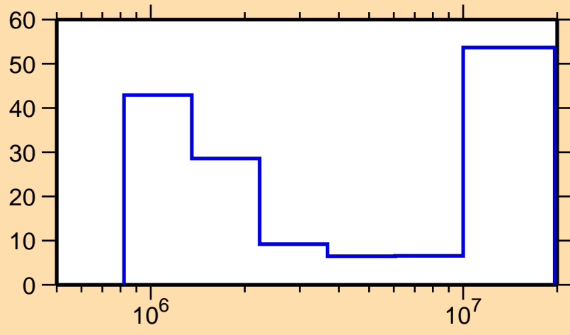
\Delta\sigma/\sigma vs. E for ^{157}\text{Tb}(n,n\text{cont.})
