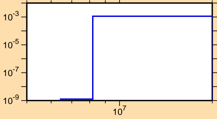
\sigma vs. E for ^{157}\text{Tb}(n,np)
