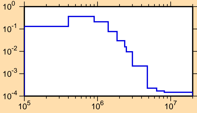
\sigma vs. E for ^{157}\text{Tb}(n,n_2)
