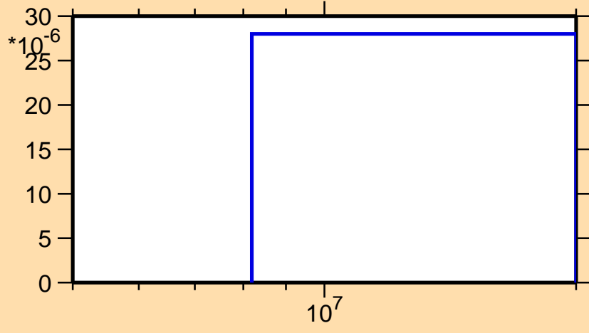
\sigma vs. E for ^{157}\text{Tb}(n,t)
