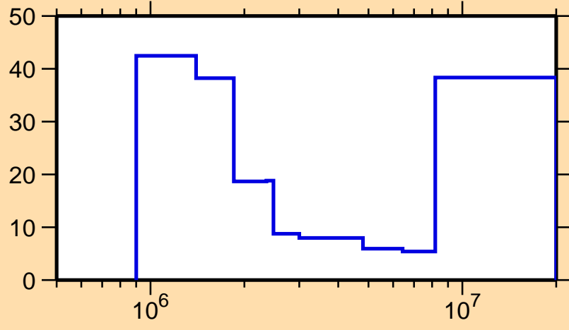
\Delta\sigma/\sigma vs. E for ^{157}\text{Tb}(n,n\text{cont.})
