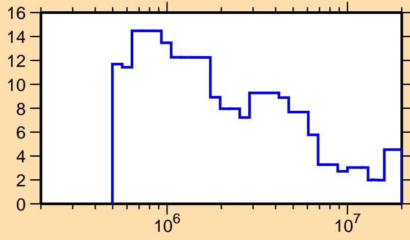
\Delta\sigma/\sigma vs. E for ^{158}\text{Tb}(n,\text{tot.})
