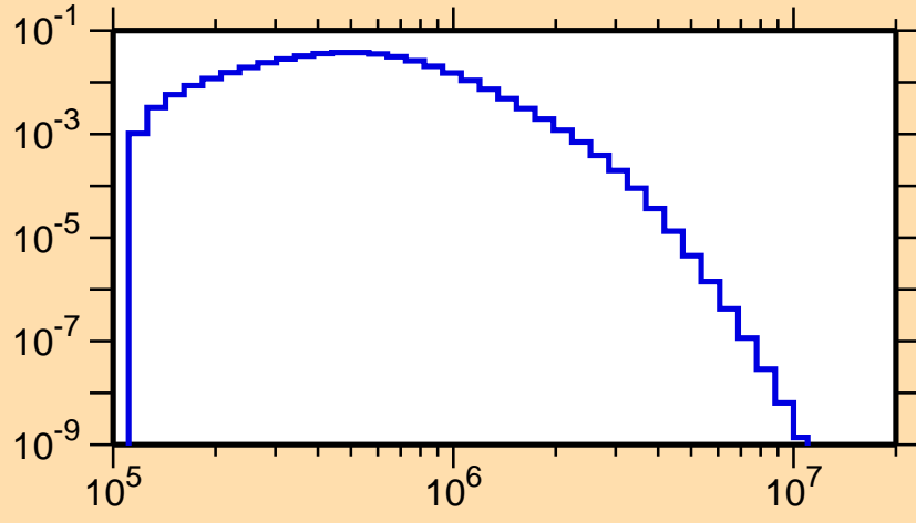
\sigma vs. E for ^{158}\text{Tb}(n,n_3)
