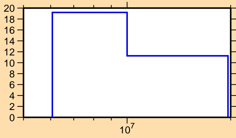
\Delta\sigma/\sigma vs. E for ^{158}\text{Tb}(n,2n)
