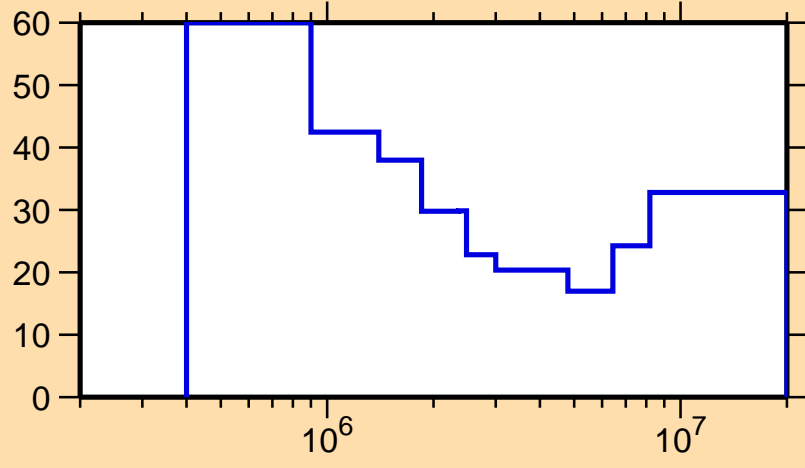
\Delta\sigma/\sigma vs. E for ^{158}\text{Tb}(n,n\text{cont.})
