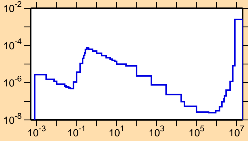
\sigma vs. E for ^{158}\text{Tb}(n,\alpha)
