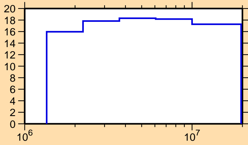
\Delta\sigma/\sigma vs. E for ^{159}\text{Tb}(n,n_1)
