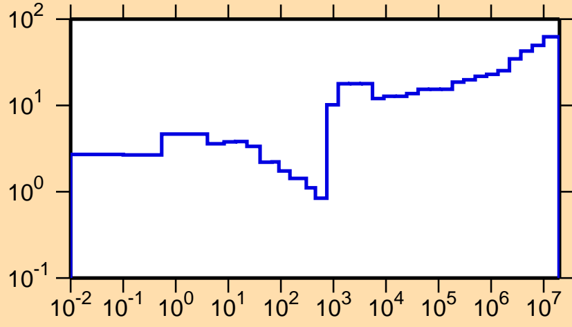
\Delta\sigma/\sigma vs. E for ^{159}\text{Tb}(n,\gamma)
