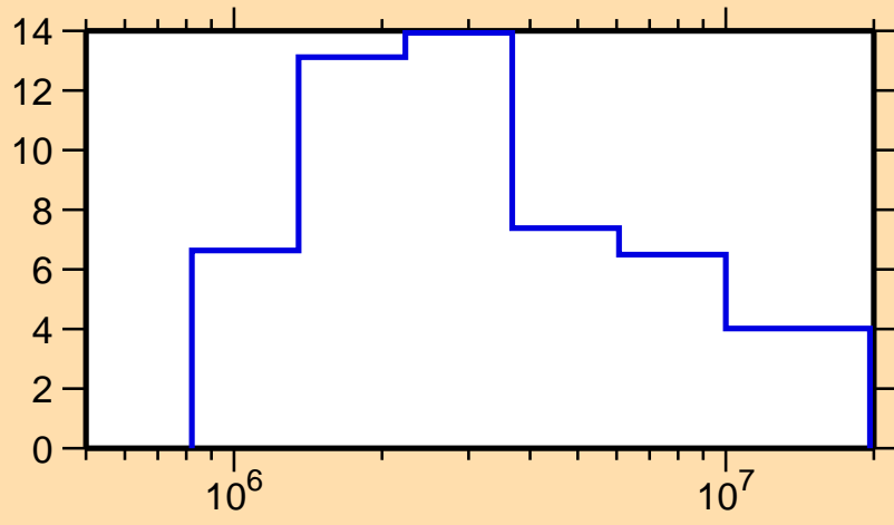
\Delta\sigma/\sigma vs. E for ^{159}\text{Tb}(n,\text{el.})
