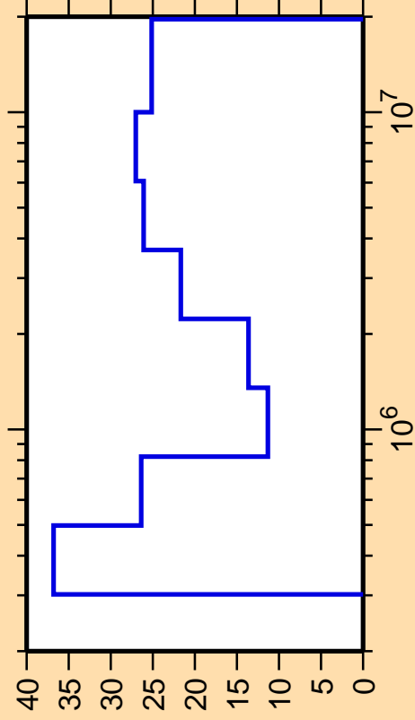
\Delta\sigma/\sigma vs. E for ^{159}\text{Tb}(n,n_4)
