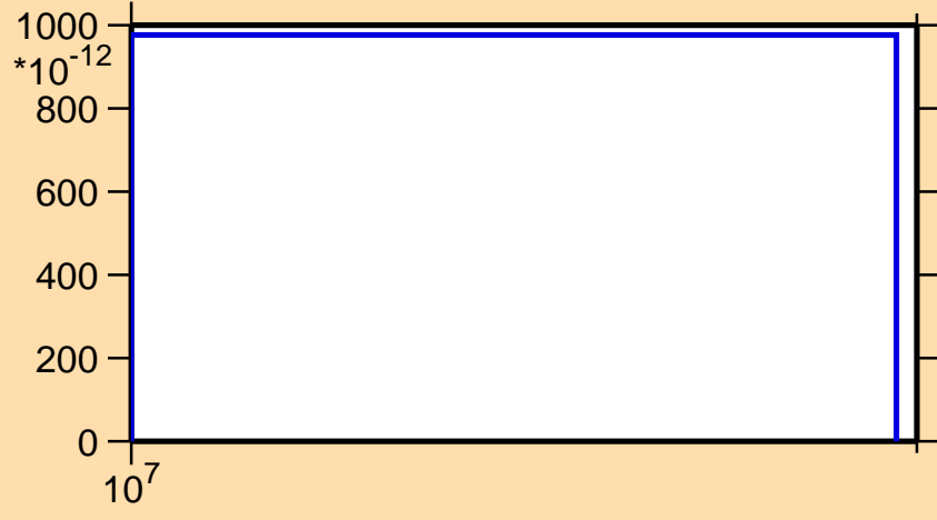
\sigma vs. E for ^{159}\text{Tb}(n,2np)
