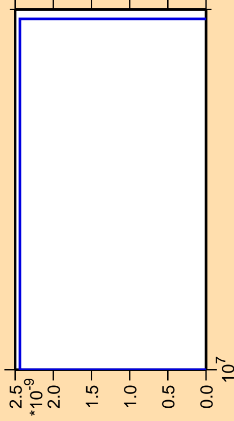
\Delta\sigma/\sigma vs. E for ^{159}\text{Tb} (mt 11)
