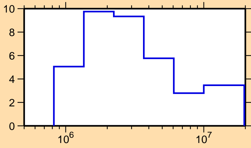
\Delta\sigma/\sigma vs. E for ^{159}\text{Tb}(n,\text{tot.})
