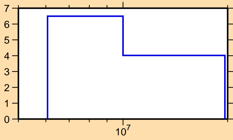
\Delta\sigma/\sigma vs. E for ^{159}\text{Tb}(n,\text{el.})
