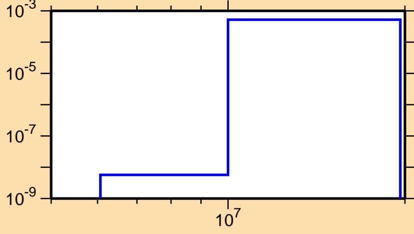
\sigma vs. E for ^{159}\text{Tb}(n,d)
