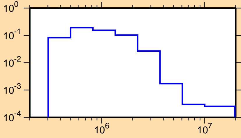
\sigma vs. E for ^{159}\text{Tb}(n,n_4)
