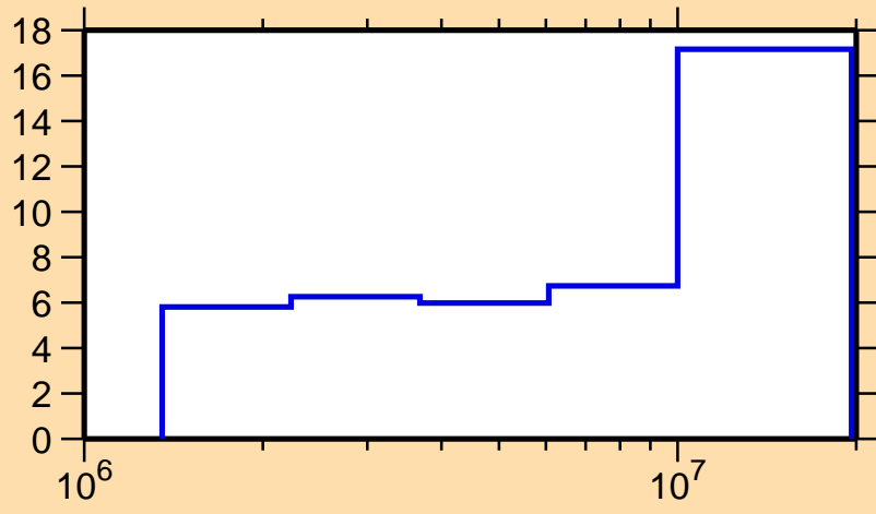
\Delta\sigma/\sigma vs. E for ^{159}\text{Tb}(n,\text{inel.})
