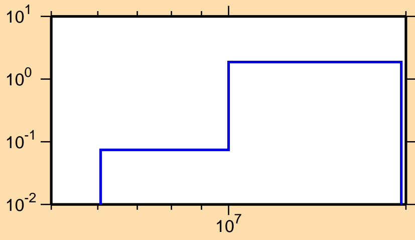
\sigma vs. E for ^{159}\text{Tb}(n,2n)
