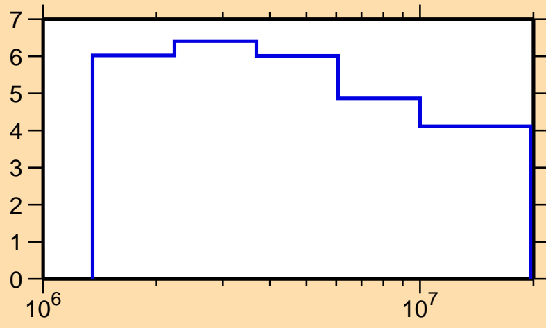
\Delta\sigma/\sigma vs. E for ^{159}\text{Tb}(n,\text{nonel.})
