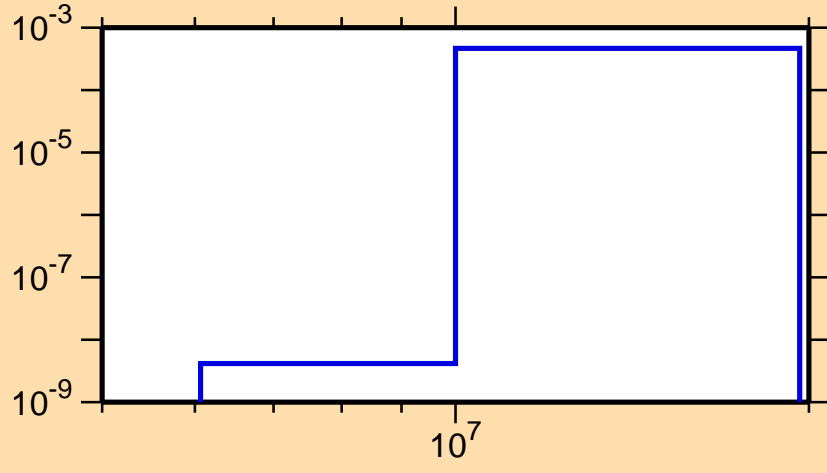
\sigma vs. E for ^{159}\text{Tb}(n,np)
