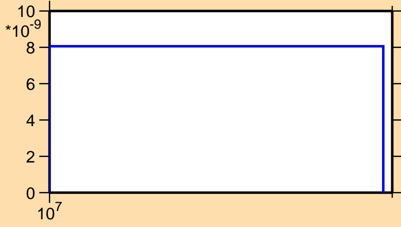
\sigma vs. E for ^{159}\text{Tb}(n,nt)
