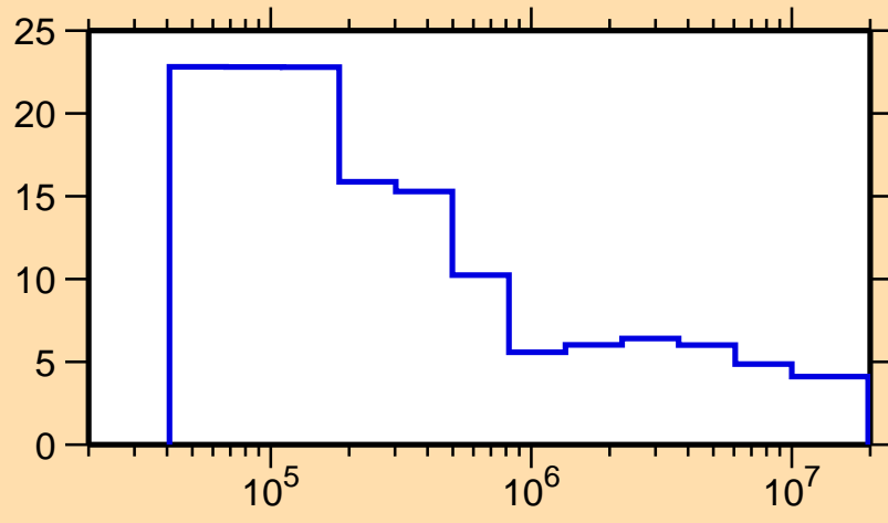
\Delta\sigma/\sigma vs. E for ^{159}\text{Tb}(n,\text{nonel.})
