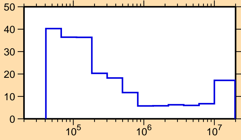
\Delta\sigma/\sigma vs. E for ^{159}\text{Tb}(n,\text{inel.})
