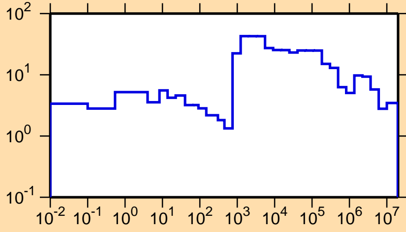
\Delta\sigma/\sigma vs. E for ^{159}\text{Tb}(n,\text{tot.})
