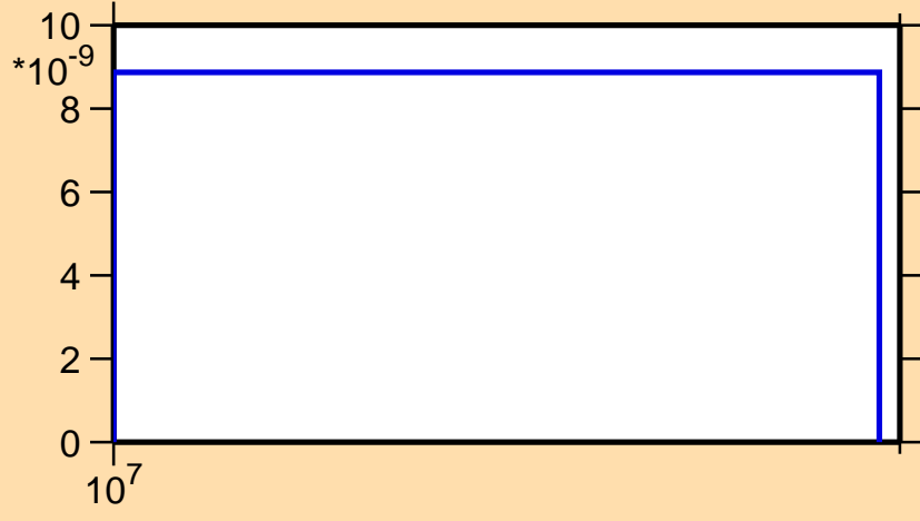
\sigma vs. E for ^{159}\text{Tb}(n,\text{nd})
