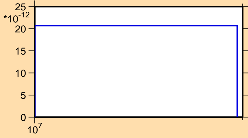
\sigma vs. E for ^{159}\text{Tb}(n,\text{He3})
