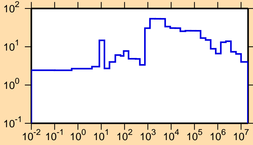
\Delta\sigma/\sigma vs. E for ^{159}\text{Tb}(n,\text{el.})
