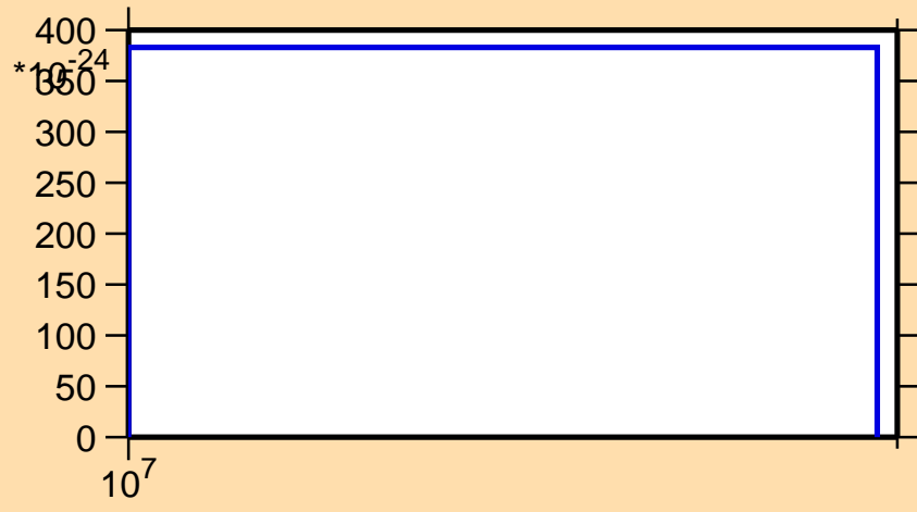
\sigma vs. E for ^{159}\text{Tb} (mt 11)
