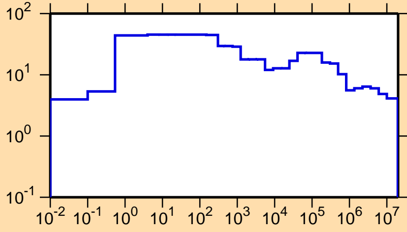
\Delta\sigma/\sigma vs. E for ^{159}\text{Tb}(n,\text{nonel.})
