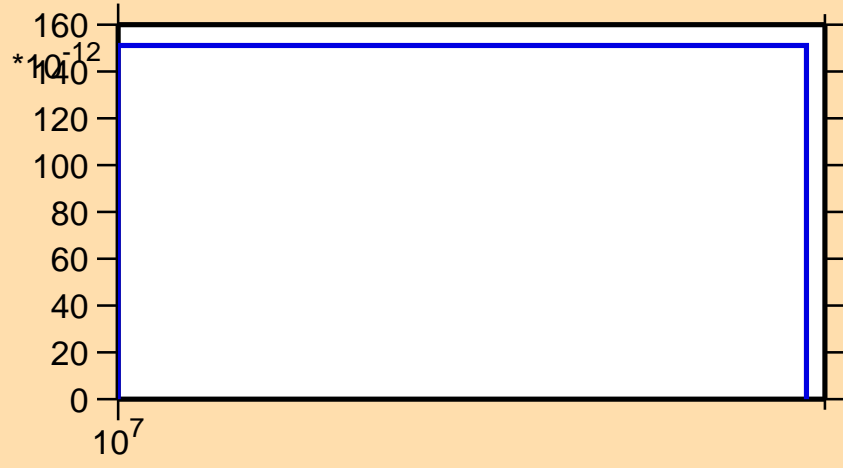
\sigma vs. E for ^{159}\text{Tb}(n,2n\alpha)
