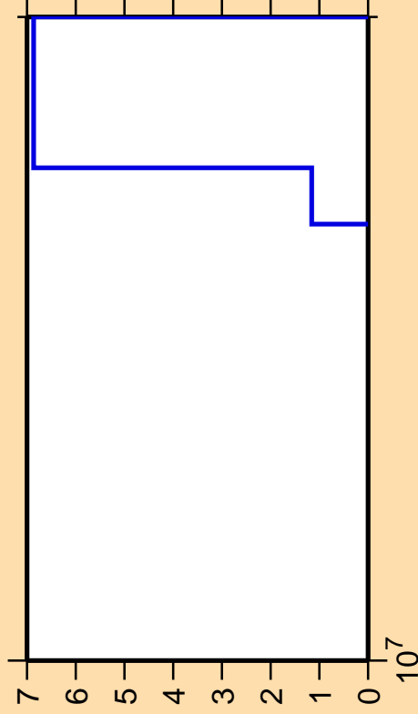
\Delta\sigma/\sigma vs. E for ^{160}\text{Tb}(n,p\alpha)
