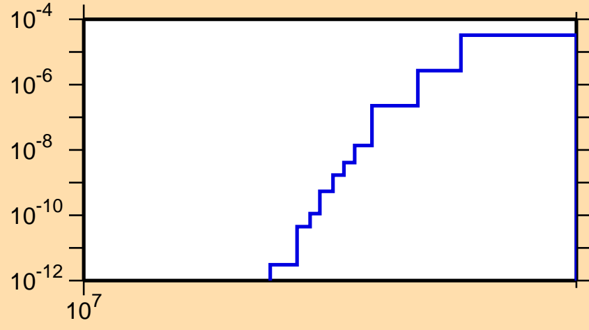
\sigma vs. E for ^{160}\text{Tb}(n,\text{nd})
