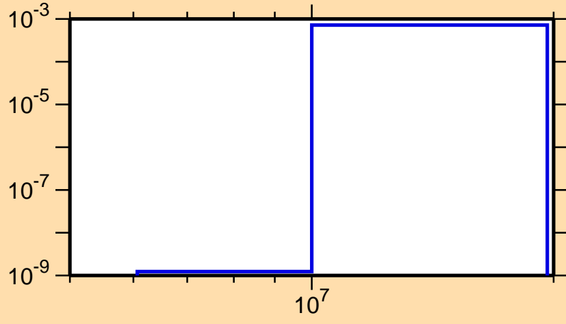
\sigma vs. E for ^{160}\text{Tb}(n,np)
