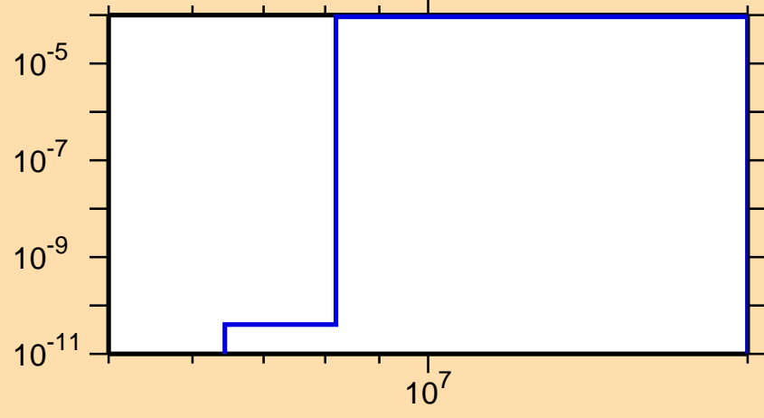
\sigma vs. E for ^{160}\text{Tb}(n,n\alpha)
