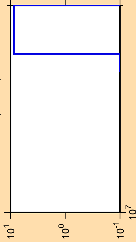
\Delta\sigma/\sigma vs. E for ^{161}\text{Tb}(n,\text{He3})
