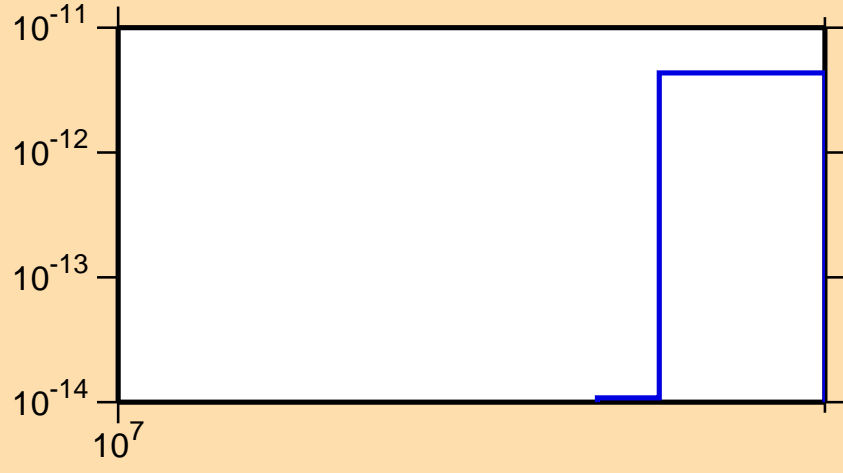
\sigma vs. E for ^{161}\text{Tb}(n,\text{He3})
