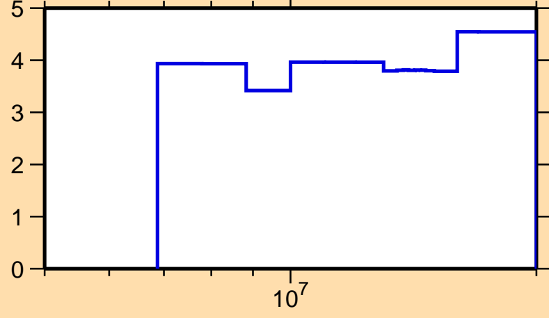
\Delta\sigma/\sigma vs. E for ^{161}\text{Tb}(n,\text{tot.})
