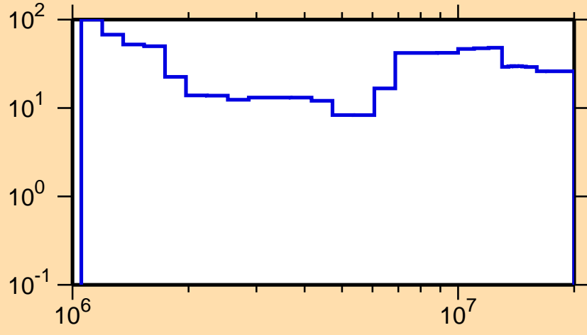
\Delta\sigma/\sigma vs. E for ^{161}\text{Tb}(n,n\text{cont.})
